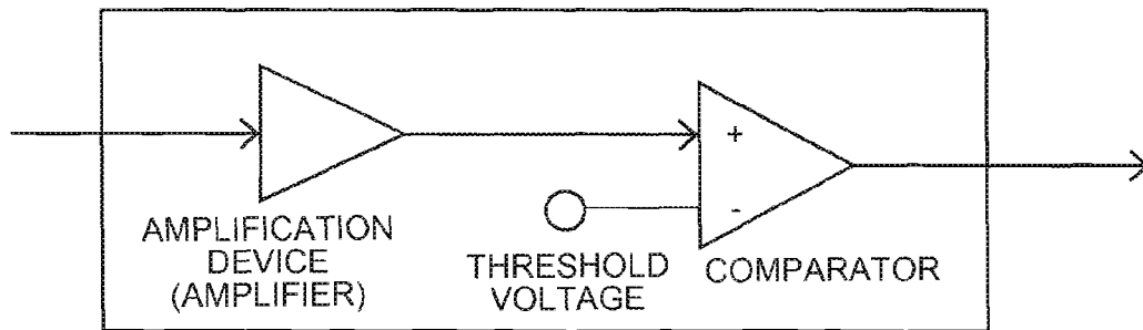
PD OUTPUT DETECTING UNIT
