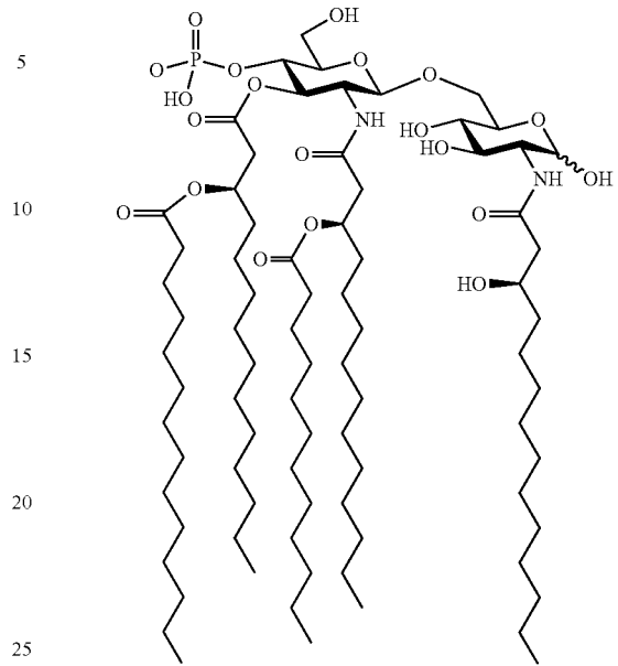
Formula (IV)
