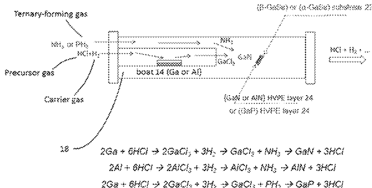
Heteroepitaxy of GaN or AlN on β-GaSe, and GaP on α-GaSe
