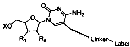
Cytidine C5-linker
