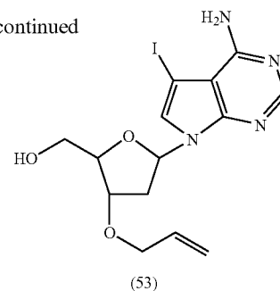
3'-O-Allyl-7-deaza-7-iodo-2'-deoxyadenosine (53)
