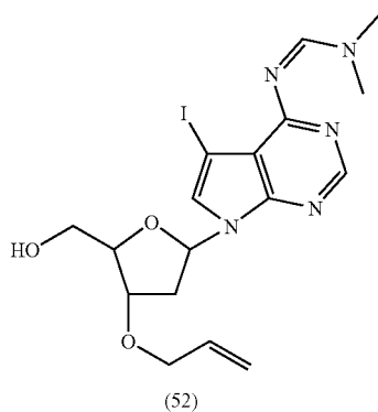
3'-O-Allyl-7-deaza-6-N,N-dimethylformidine-7-iodo-2'-deoxyadenosine (52)
