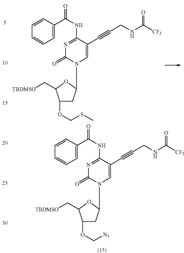
4-N-Benzoyl-5'-O-(tert-butyl dimethylsilyl)-3'-O-azidomethyl-5-[3-(2,2,2-trifluoroacetamido)-prop-1-ynyl]-2'-deoxycytidine (15)
