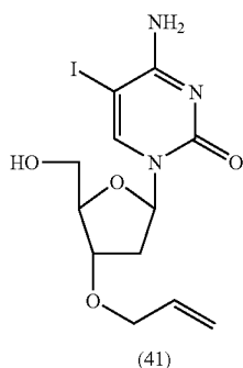
3'-O-Allyl-5-iodo-2'-deoxycytidine (41)
