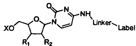
Cytidine N4-linker
