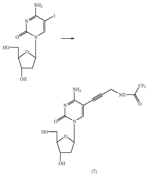
5-[3-(2,2,2-Trifluoroacetamido)-prop-1-ynyl]-2'-deoxyribose (7)
