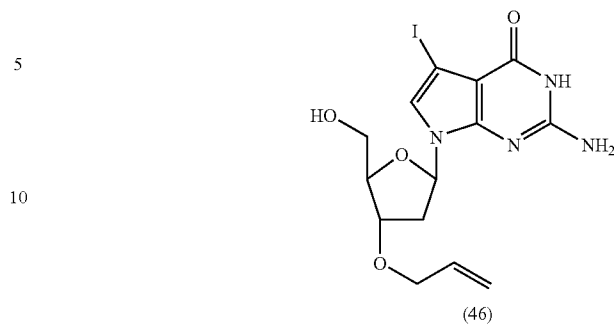
3'-O-Allyl-5'-O-(tert-butyldimethylsilyl)-7-deaza-7-iodo-2'-deoxyguanosine (46)
