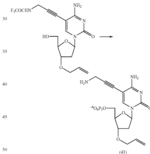
3'-O-Allyl-5-(3-amino-prop-1-ynyl)-5'-O-triphosphate-2'-deoxycytidine (43)
