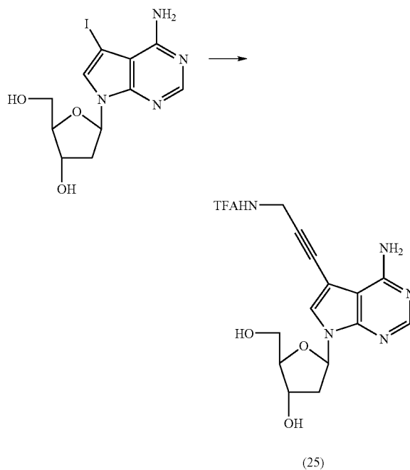
7-Deaza-7-[3-(2,2,2-trifluoroacetamido)prop-1-ynyl]-2'-deoxyadenosine (25)
