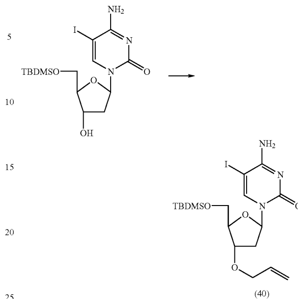
3'-O-Allyl-5'-O-(tert-butyldimethylsilyl)-5-iodo-2'-deoxycytidine (40)
