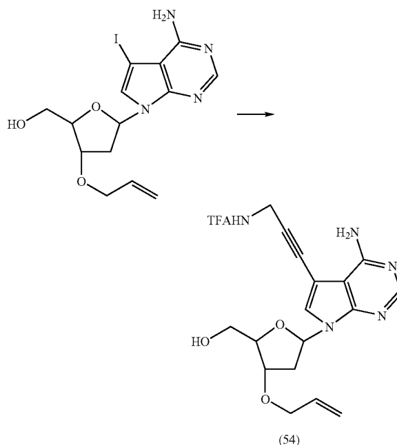
3'-O-Allyl-7-deaza-7-[3-(2,2,2-trifluoroacetamide)]-2'-deoxyadenosine (54)
