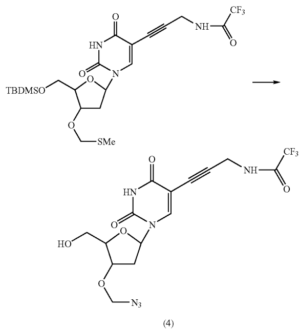
3'-O-Azidomethyl-5-[3-(2,2,2-trifluoroacetamido)-prop-1-ynyl]-2'-deoxyuridine (4)
