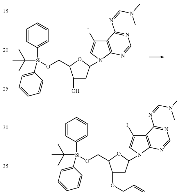
7-Deaza-5'-O-diphenylsilyl-7-iodo-2'-deoxyadenosine (49)
