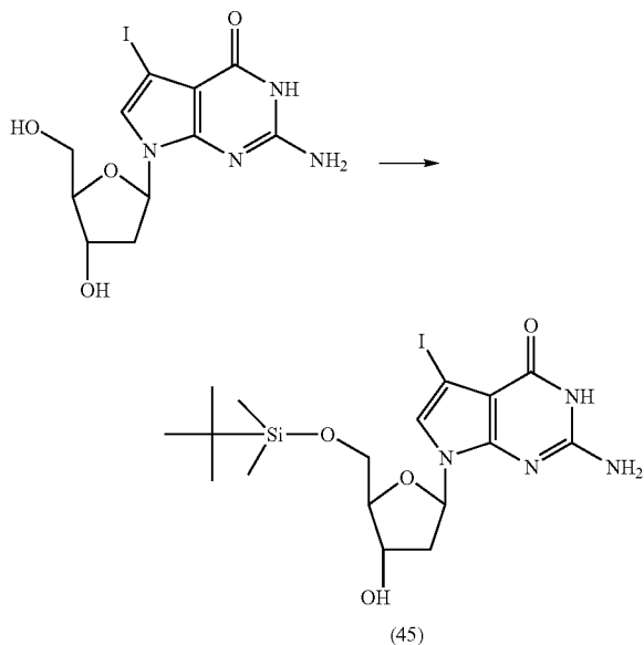
5'-O-(tert-Butyldimethylsilyl)-7-deaza-7-iodo-2'-deoxyguanosine (45)
