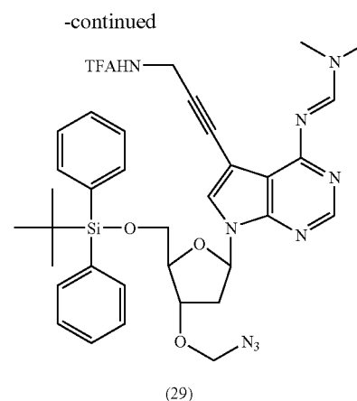
3'-O-Azidomethyl-5'-O-(tert-butyl diphenylsilyl)-7-deaza-4-N,N-dimethylformadin-7-[3-(2,2,2-trifluoroacetamido)-prop-1-ynyl]-2'-deoxyadenosine (29)
