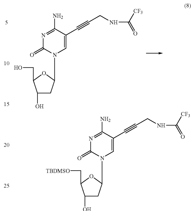
5'-O-(tert-Butyldimethylsilyl)-5-[3-(2,2,2-trifluoroacetamido)-prop-1-ynyl]-2'-deoxyribose (8)
