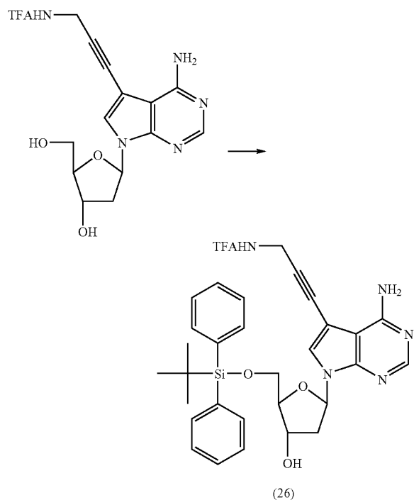
5'-O-(tert-Butyldiphenylsilyl)-7-deaza-7-[3-(2,2,2-trifluoroacetamido)-prop-1-ynyl]-2'-deoxyadenosine (26)
