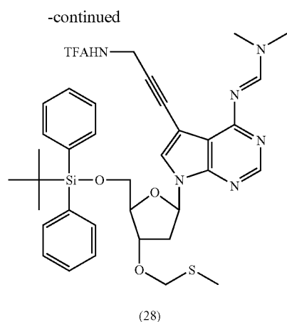
5'-O-(tert-Butyldiphenylsilyl)-7-deaza-4-N,N-dimethylformadin-3'-O-methylthiomethoxy-7-[3-(2,2,2-trifluoroacetamido)-prop-1-ynyl]-2'-deoxyadenosine (28)
