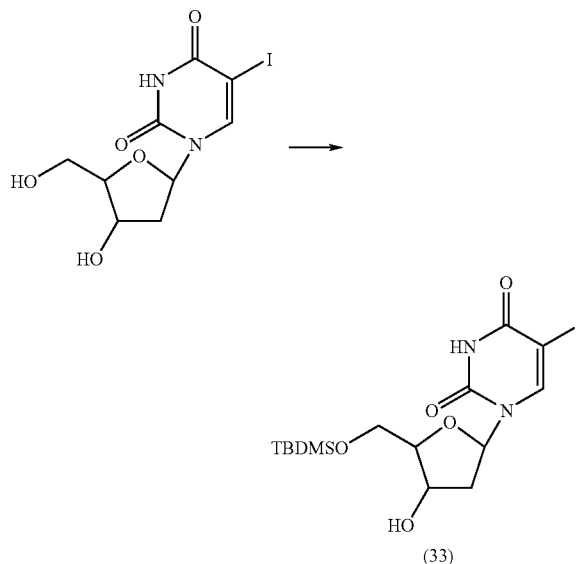
5'-O-(t-Butyldimethylsilyl)-5-iodo-2'-deoxyuridine (33)
