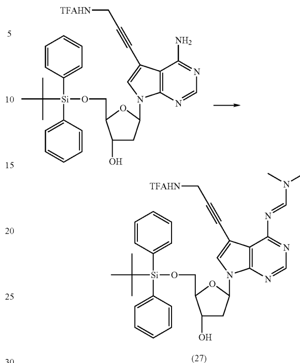
5'-O-(tert-Butyldiphenylsilyl)-7-deaza-4-N,N-dimethylformadin-7-[3-(2,2,2-trifluoroacetamido)-prop-1-ynyl]-2'-deoxyadenosine (27)
