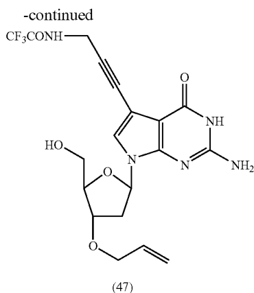
3'-O-Allyl-5'-O-(tert-butyl-dimethylsilyl)-7-deaza-7-[3-(2,2,2-trifluoroacetamido)-prop-1-ynyl]-2'-deoxyguanosine (47)
