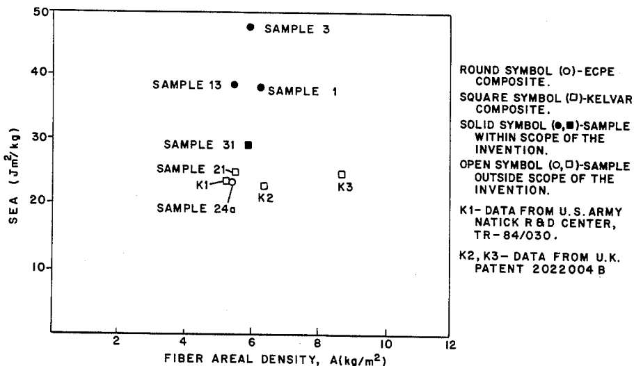
PERFORMANCE OF ECPE AND KELVAR BASED COMPOSITES
