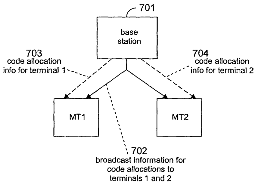
Broadcasting allocation information to terminals
