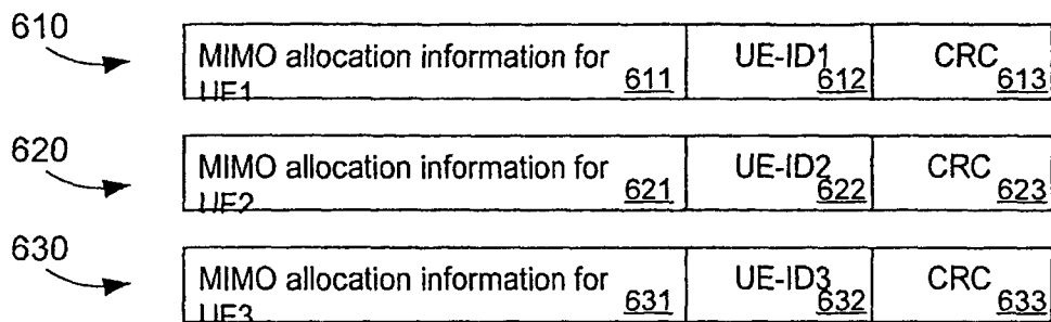
HS-SCCH structure for implicitly broadcasting allocation information
