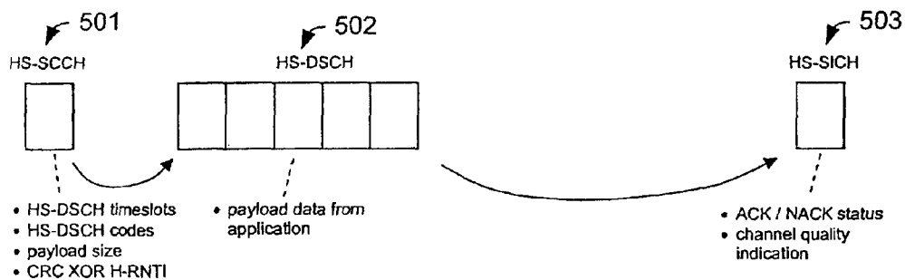
HSDPA frame structure
