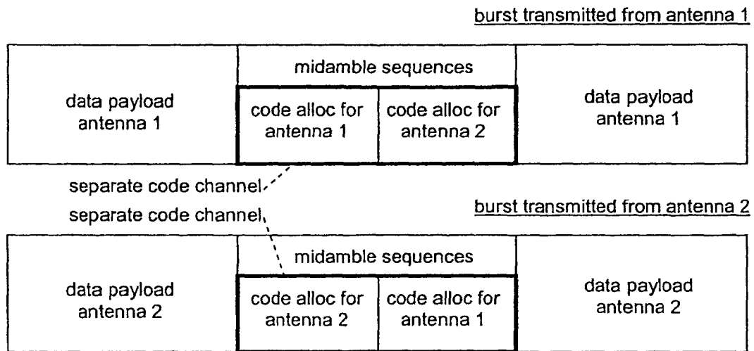
Broadcast transmission of code allocation information in midamble portion of burst
