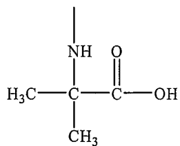
(alpha-aminoisobutyric acid)
