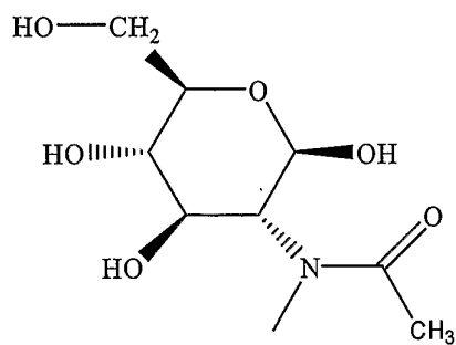
(N-acetyl glucosamine)
