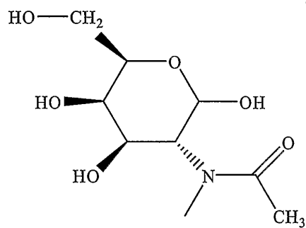
(N-acetyl galactosamine)
