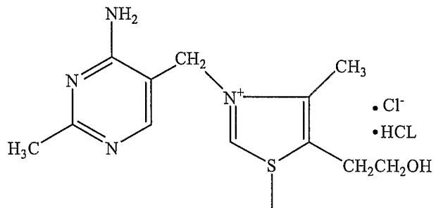
(thiamine hydrochloride)
