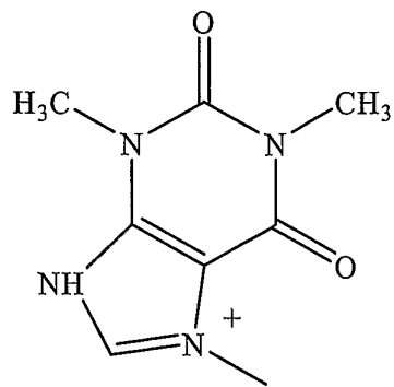
(theophylline)
