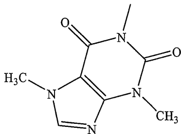
(theobromine)
