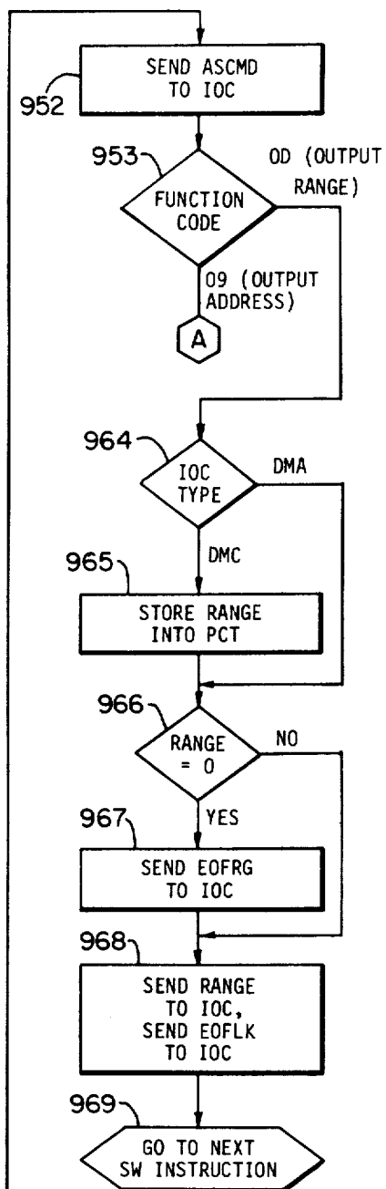
I/O INSTRUCTION FLOW CHART
