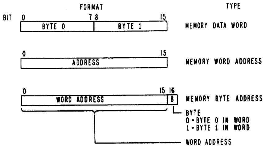
WORD AND ADDRESS FORMATS FIG. 5
