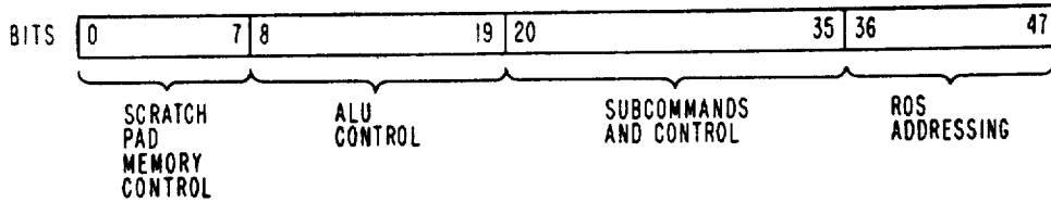
CPU FIRMWARE MICROINSTRUCTION WORD
