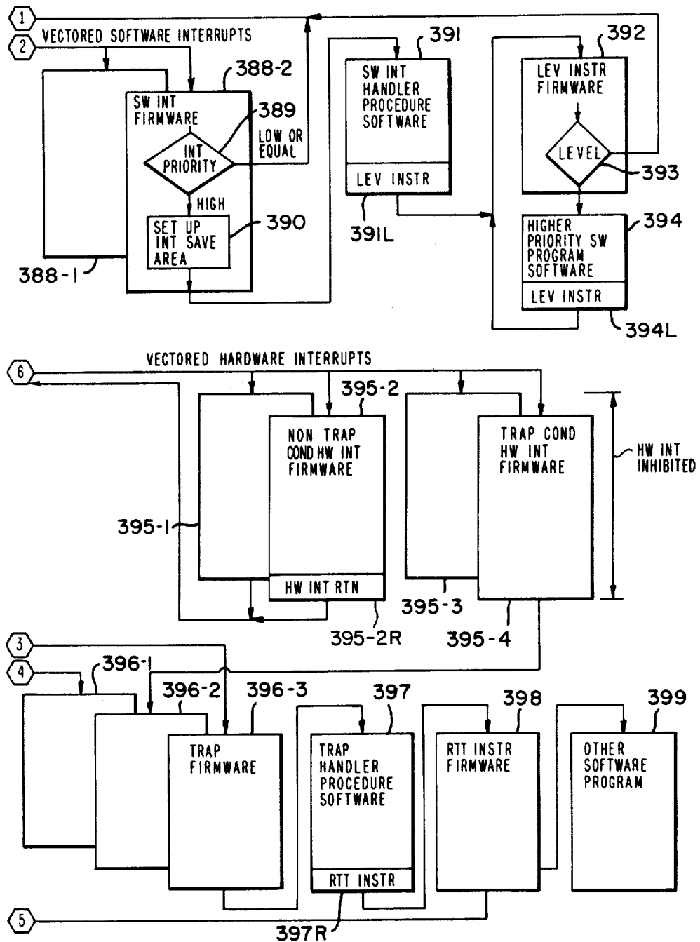
SOFTWARE INTERRUPT-TRAP-HARDWARE INTERRUPT INTERACTION
