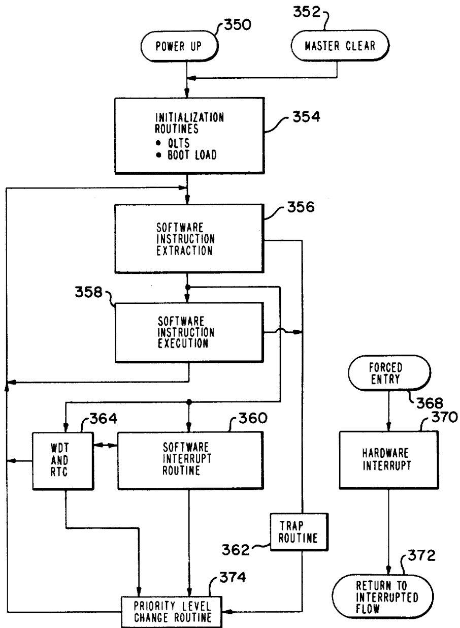
FIRMWARE FLOW OVERVIEW
