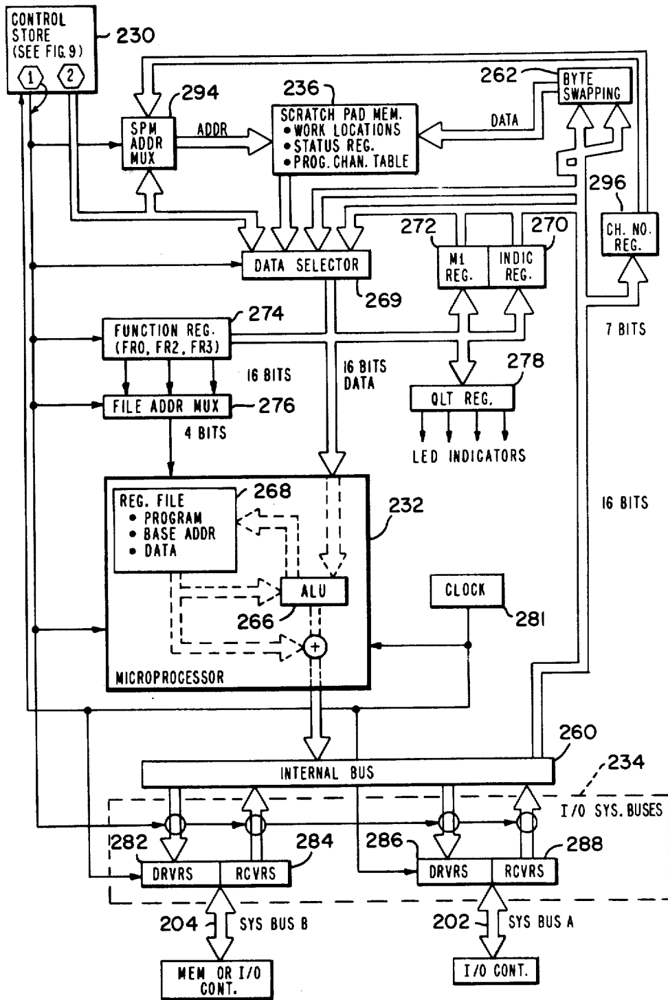
FIG. 8 CPU BLOCK DIAGRAM
