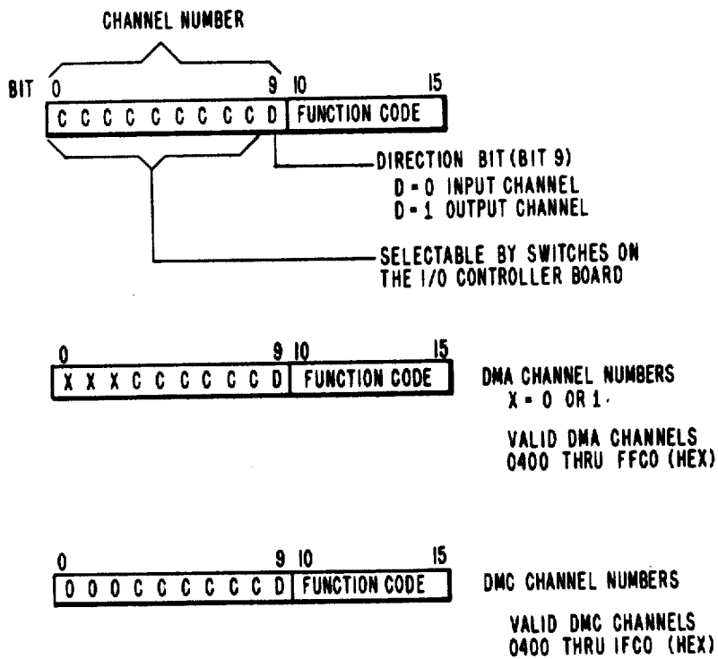
I/O SOFTWARE INSTRUCTION CONTROL WORD FORMAT
