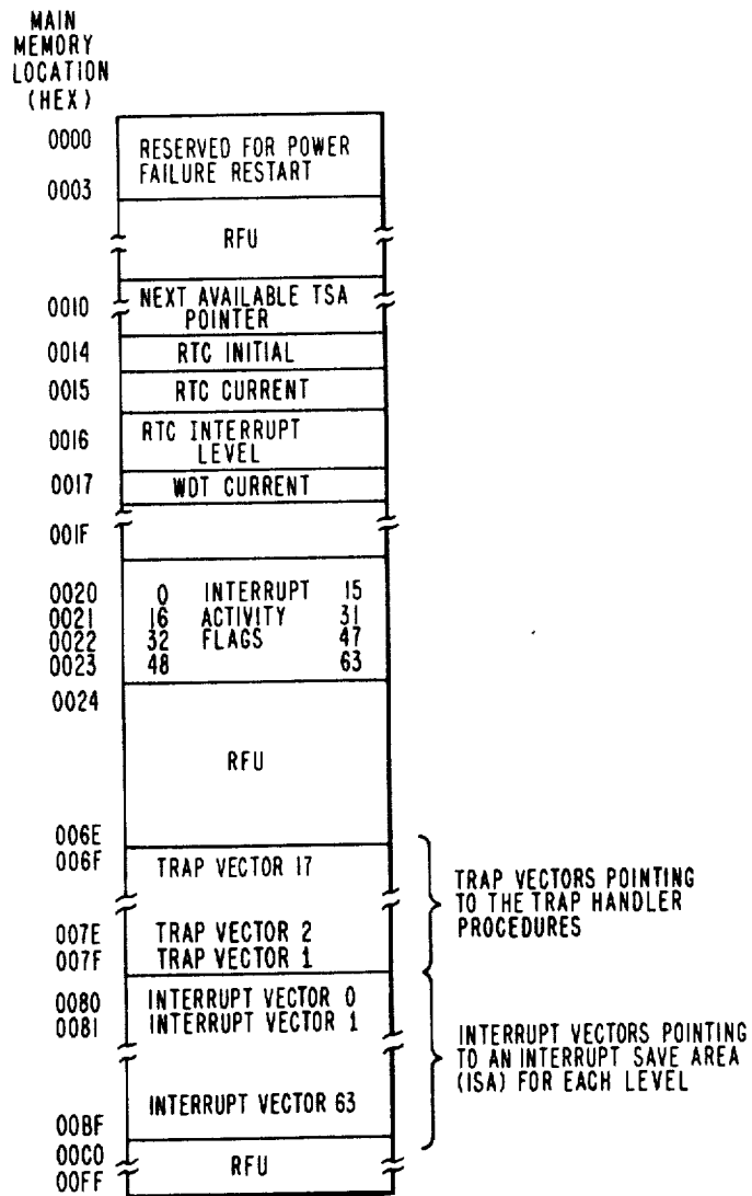
DEDICATED MAIN MEMORY LOCATIONS
