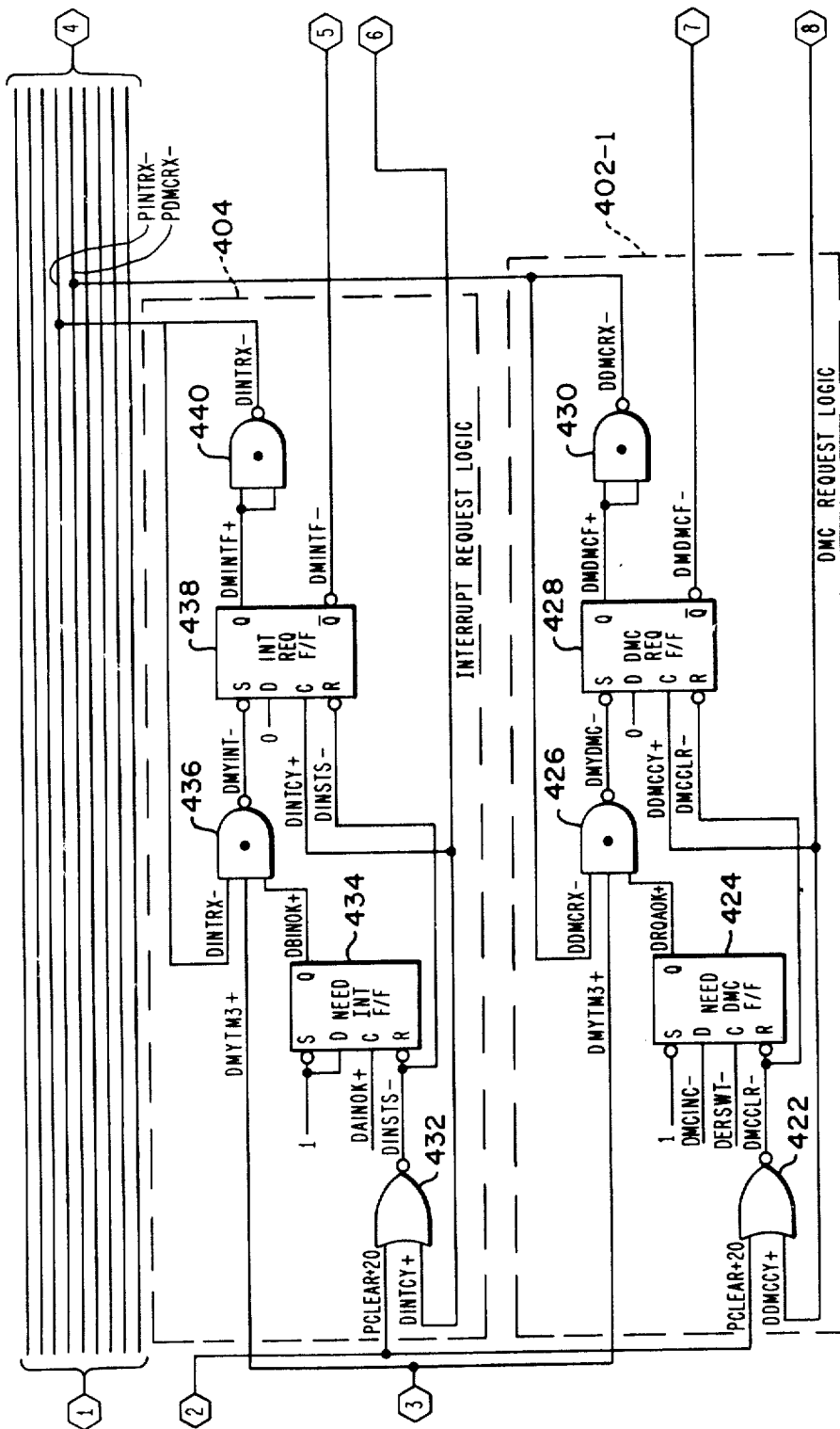
I/O CONTROLLER LOGIC FIG. 39 SHEET 2 OF 3
