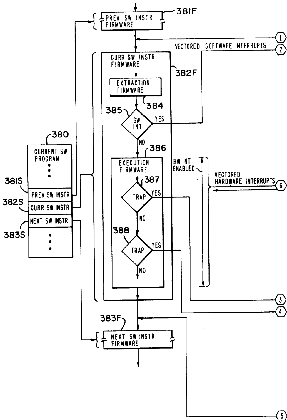
SOFTWARE INTERRUPT-TRAP-HARDWARE INTERRUPT INTERACTION
