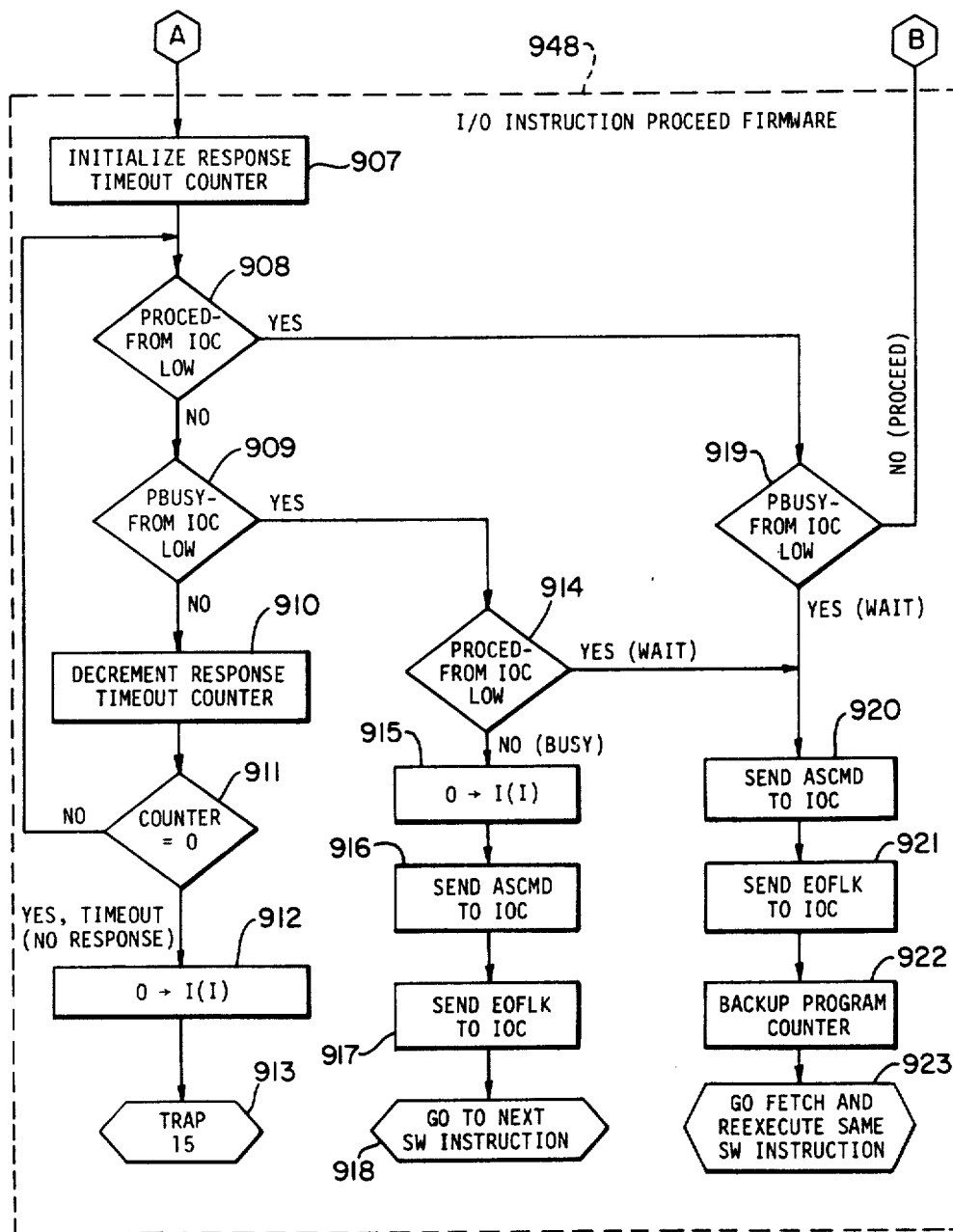
I/O INSTRUCTION FLOW CHART
