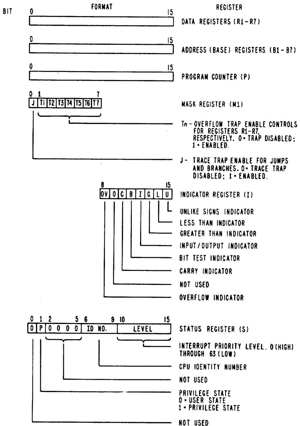
CPU REGISTERS FIG. 4
