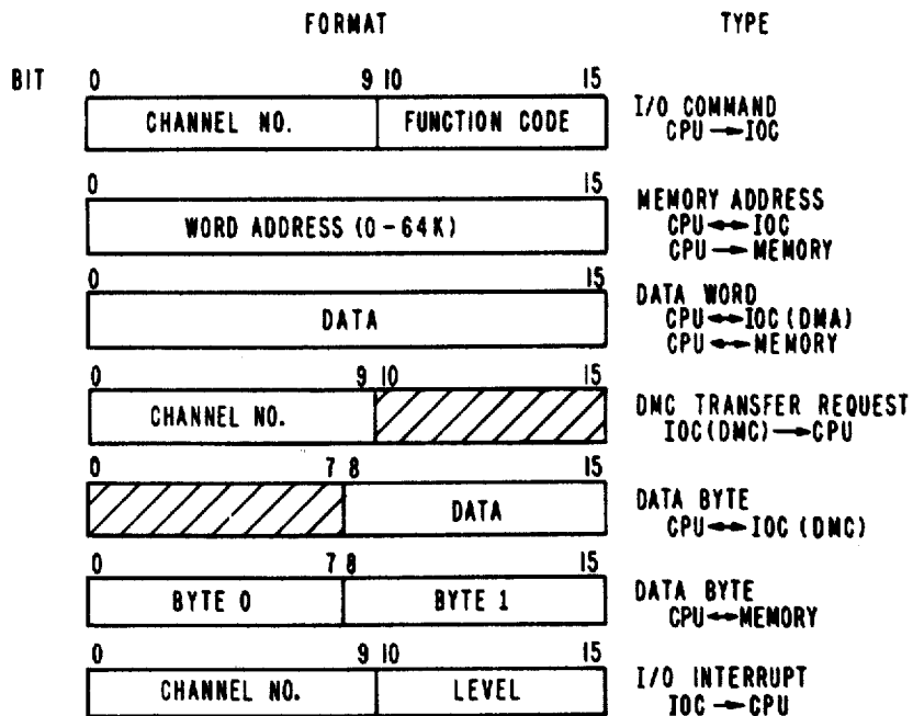
SYSTEM BUS ADDRESS / DATA LINE FORMATS FIG. 17
