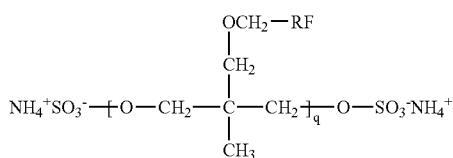
Structural Formula (3)
