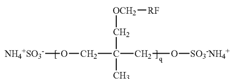
Structural Formula (3)
