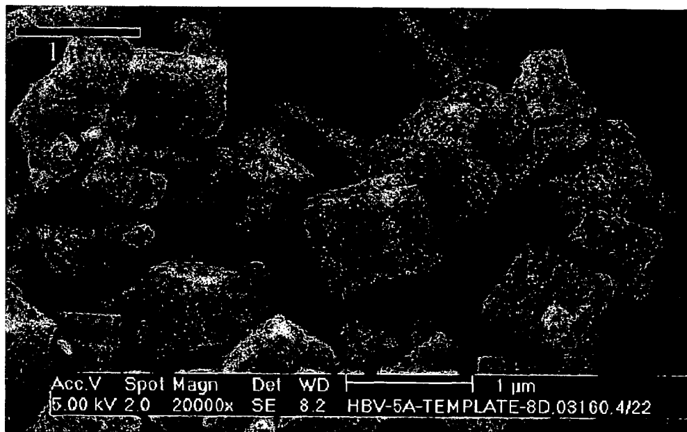
(b)MCM-68 product
