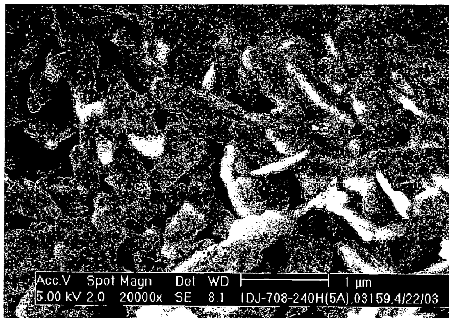
(b)MCM-68 product
