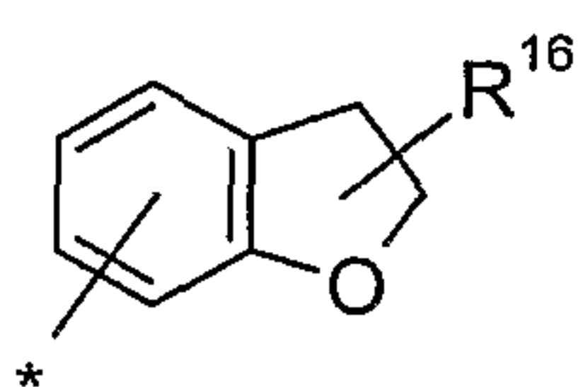
2,3-dihydrobenzofuranyl
