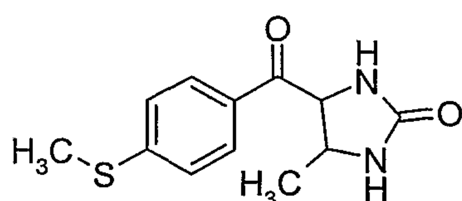
Enoximone (0.0.10)
