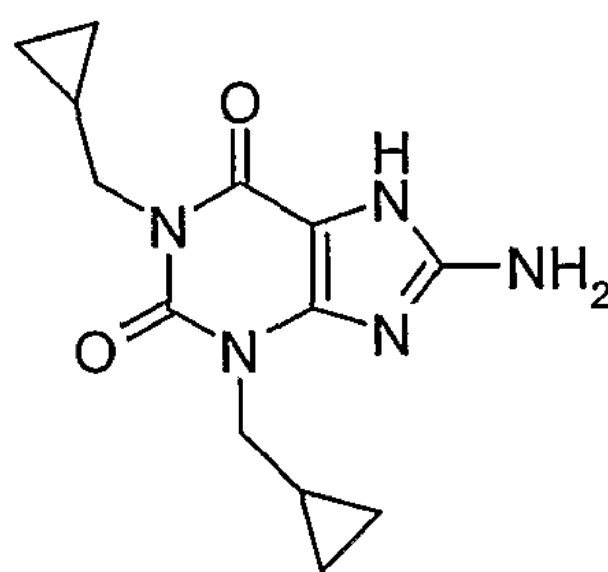
Cipamfylline
