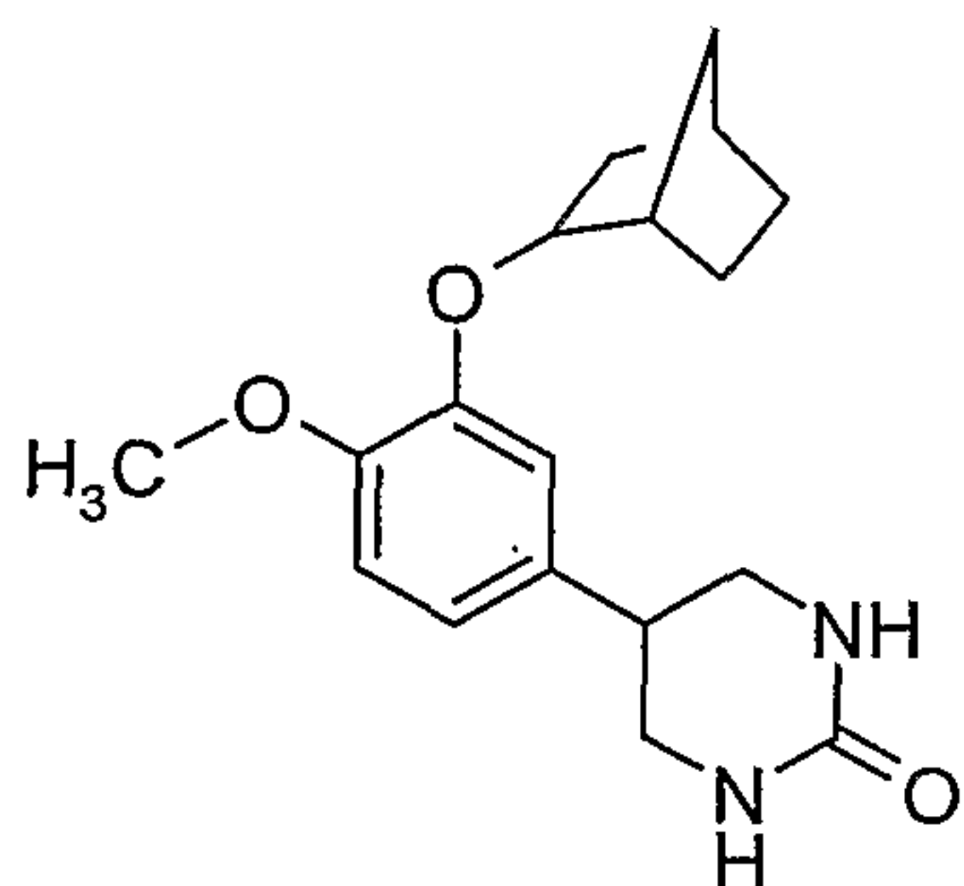
Atizoram (CP-80,633) (0.0.20)
