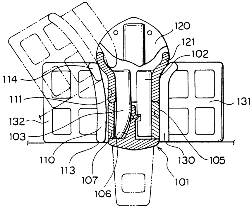
FIG. 7 (PRIOR ART)
