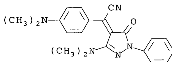
(Magenta Dye 2)
