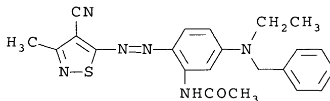
(Magenta Dye 1)
