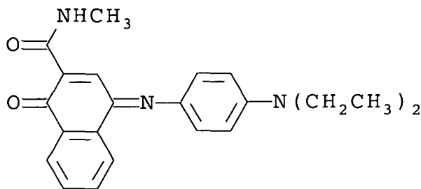
(Cyan Dye 1)
