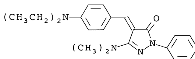
(Yellow Dye 1)
