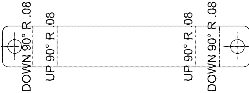
FLAT PATTERN
