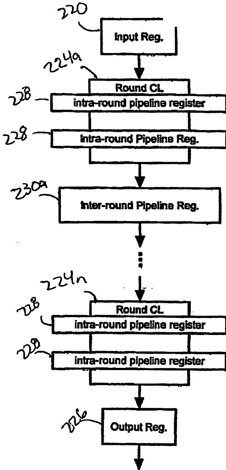
Fully pipelined encryption/decryption engine.
