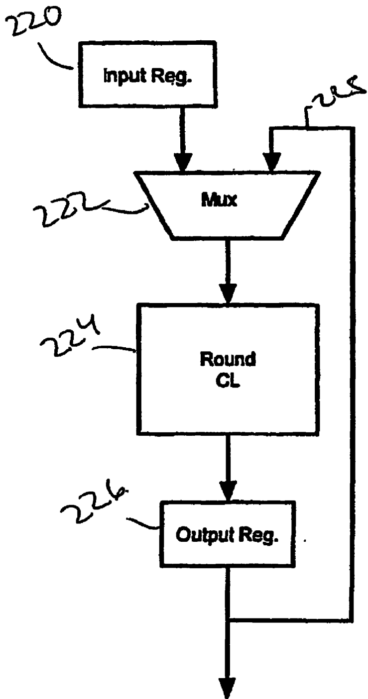
Single stage encryption/decryption engine.
