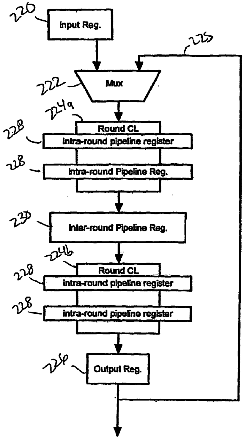
Pipelined encryption/decryption engine.
