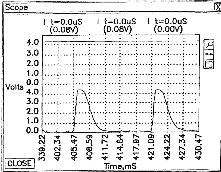
CRT photoresponse
