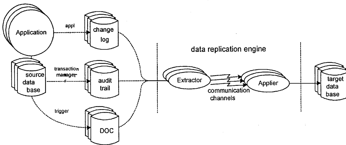
Multi-Threading
