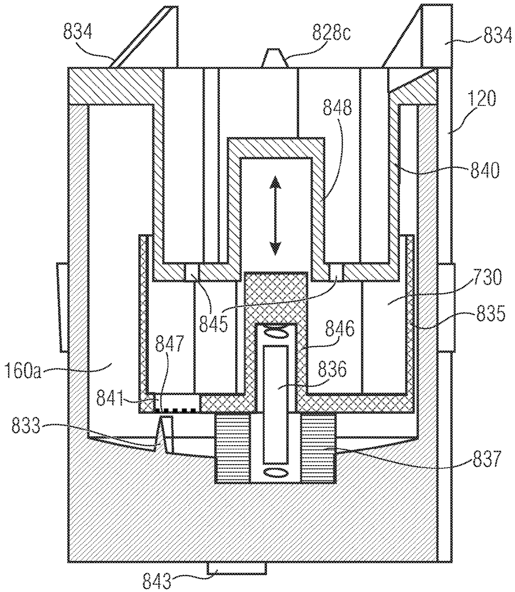
section 8CE-8CE
