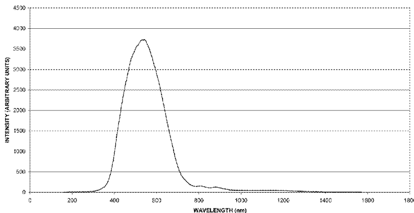
Hamamatsu Xenon Lamp Spectrum (Entire Spectrum)
