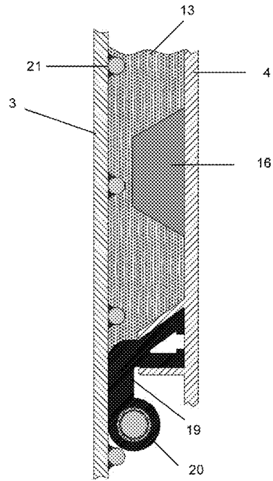
FIG. 5 (Prior Art)
