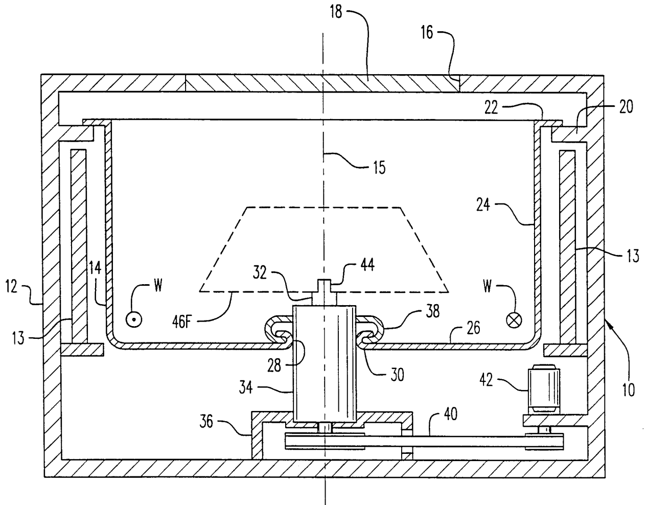
FIG. 1 (PRIOR ART)
