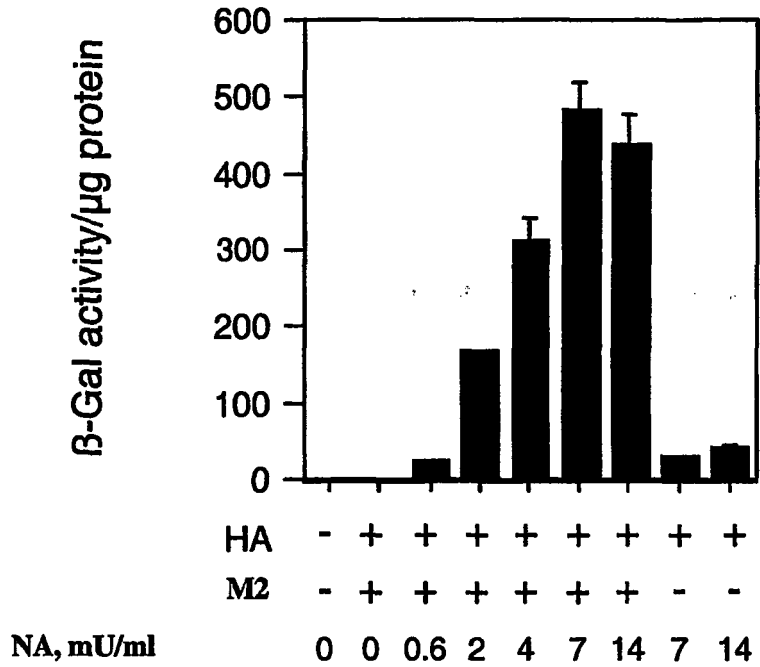
Figure 8. Comparing use of influenza NA cDNA vs bacterial NA enzyme
