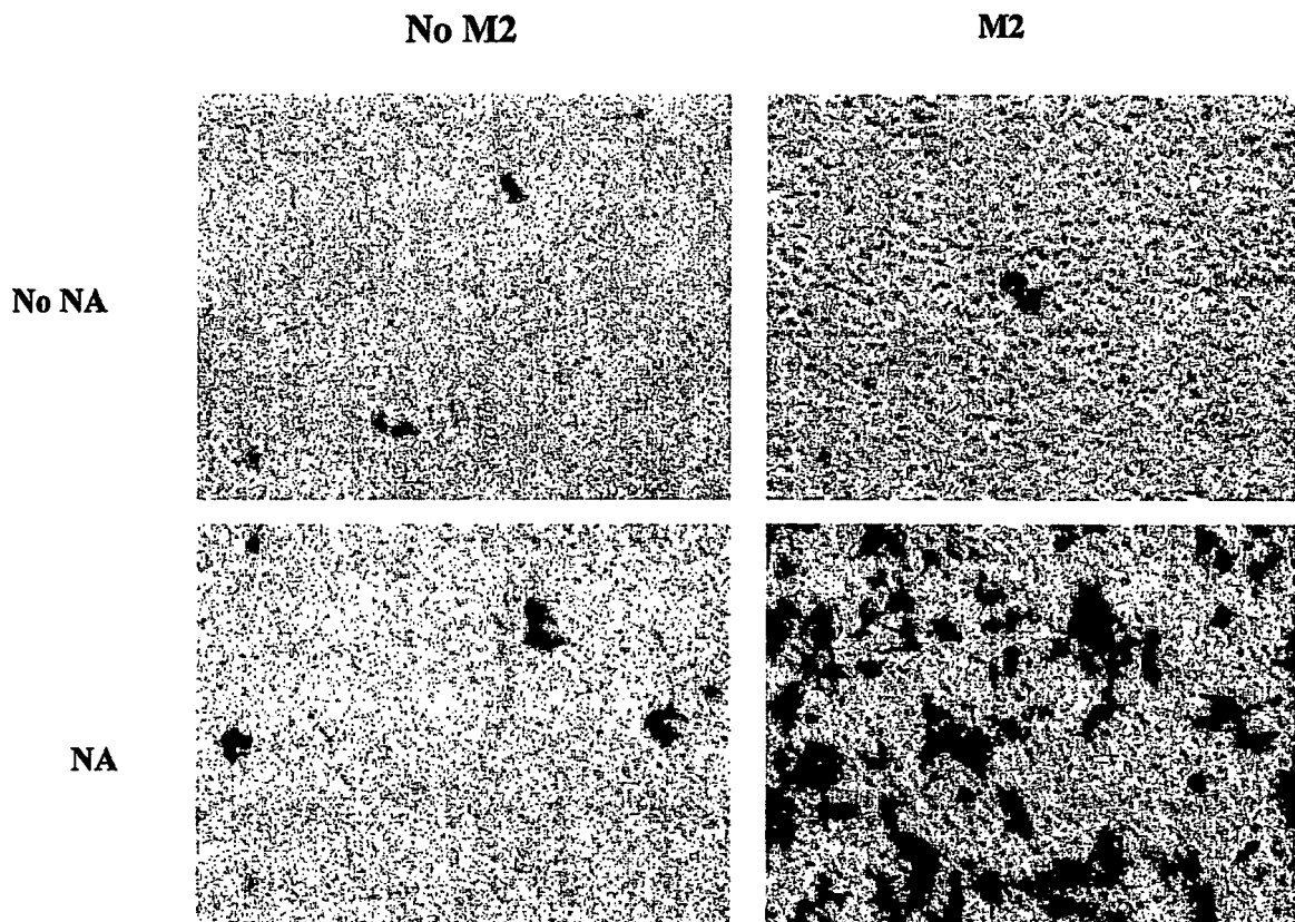
Figure 4. Gene transfer to human 293T cells by HA pseudotyped EIAV lacZ vector produced in the presence or absence of M2 expression and NA treatment.
