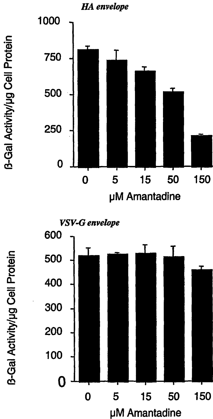
Figure 6. Role of M2 during HA-mediated ELAV vector gene transfer
