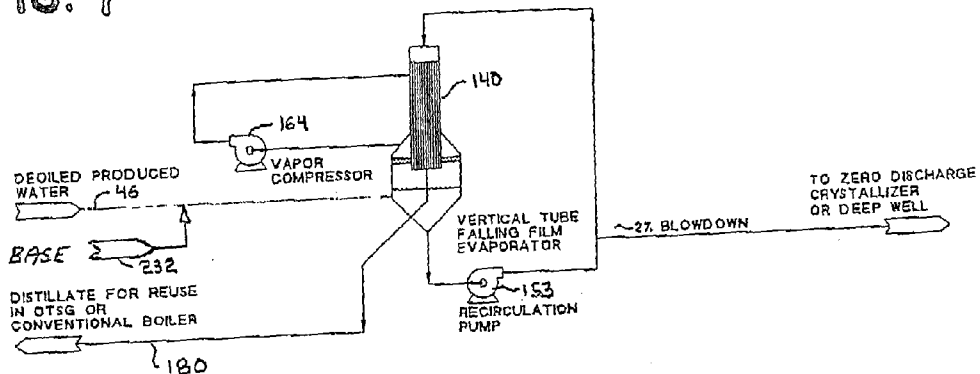
Simplified Vapor Compression Falling Film Evaporator System
