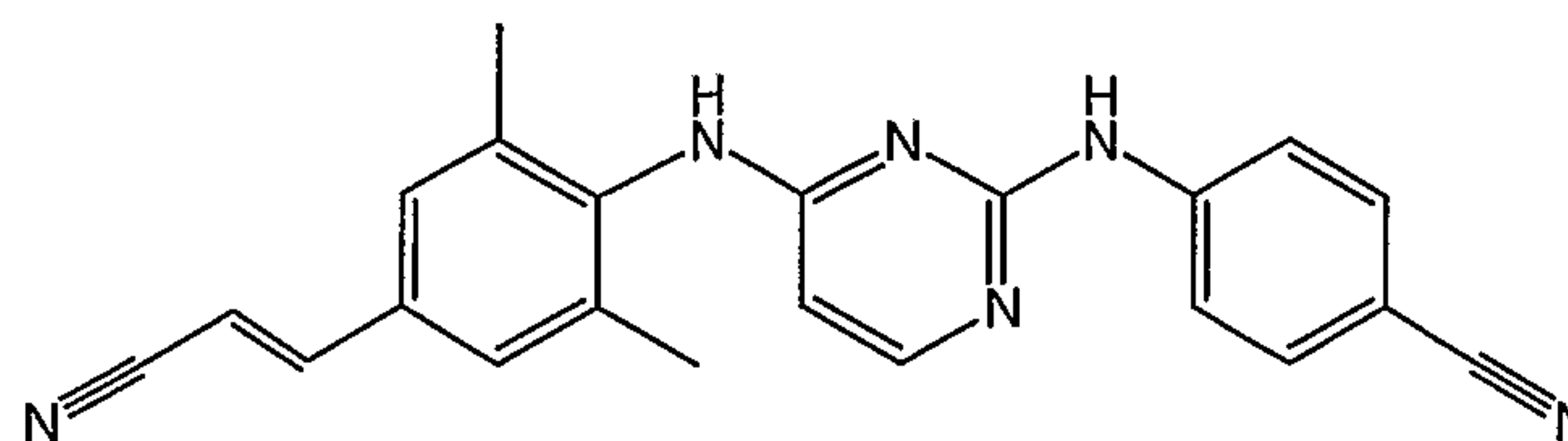
Compound 1=(E); compound 10=(Z)
