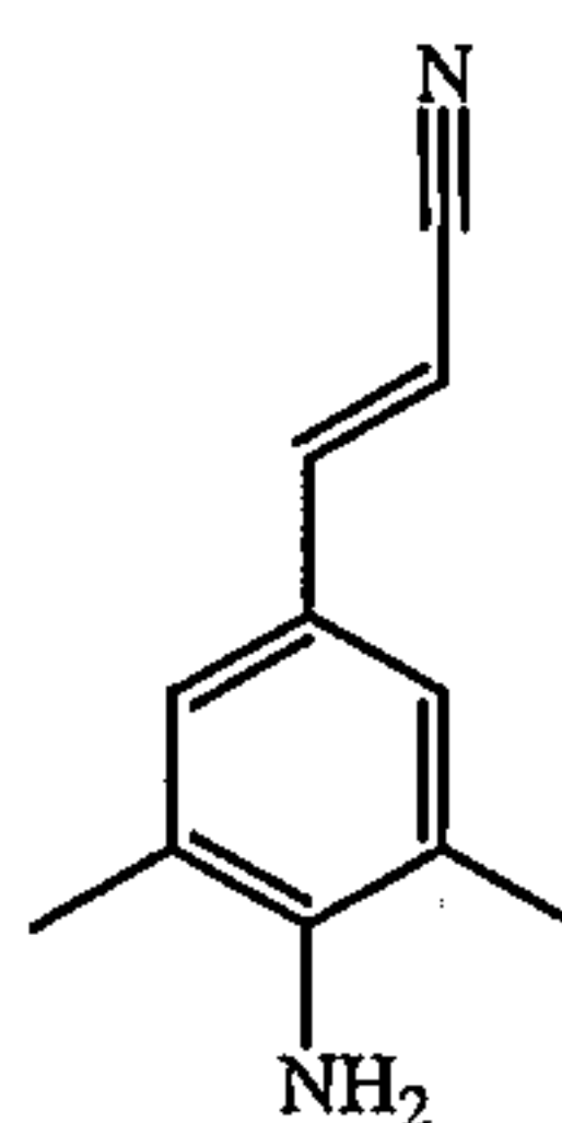
Intermediate 3
