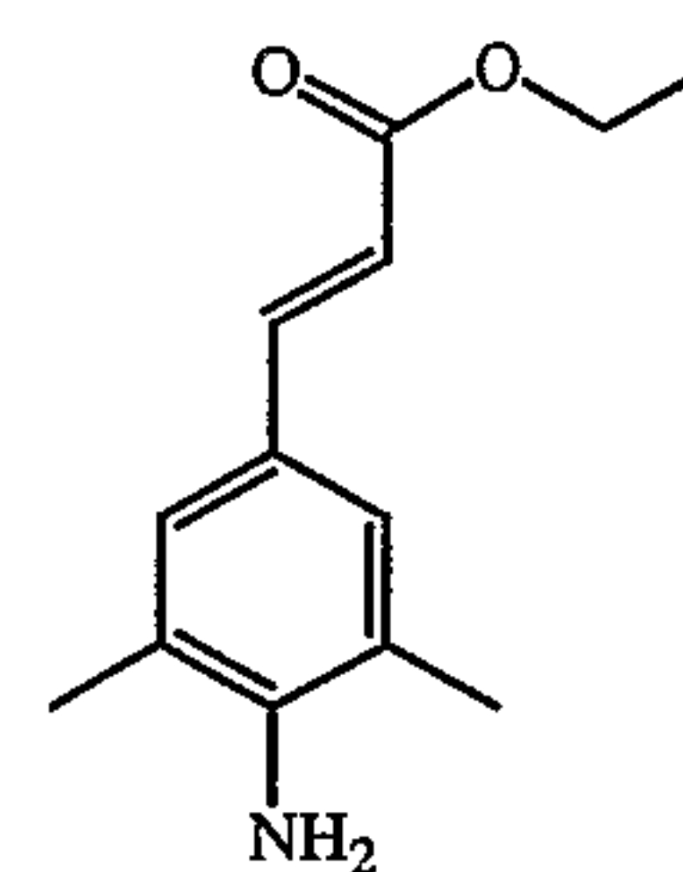
Intermediate 22
