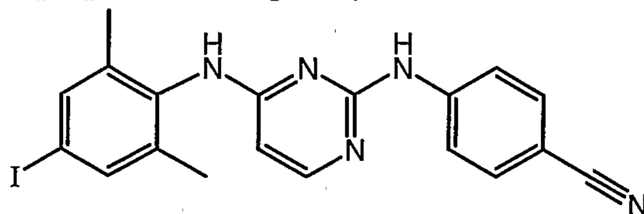
Intermediate 59
