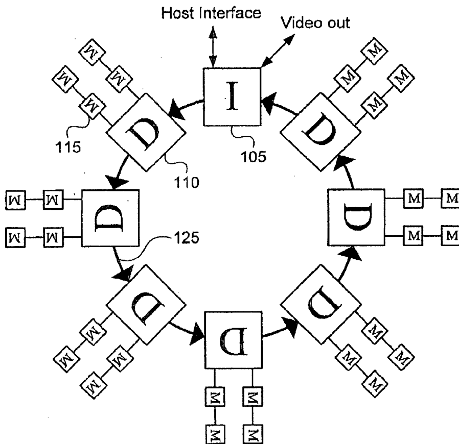
Basic Loop Architecture Interconnect
