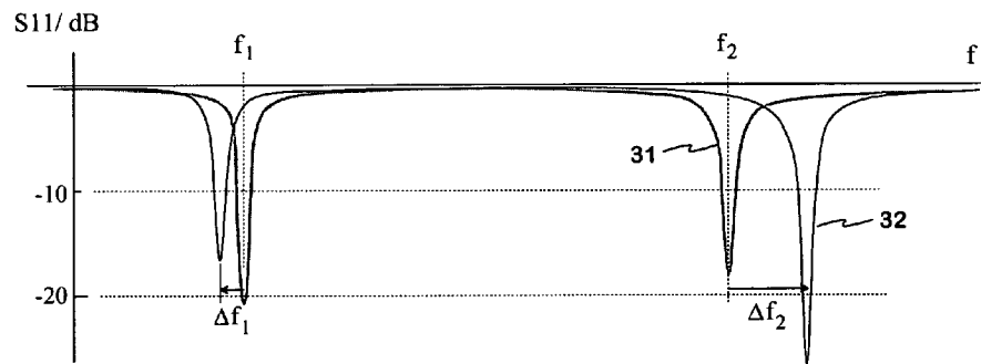
Fig. 3 PRIOR ART
