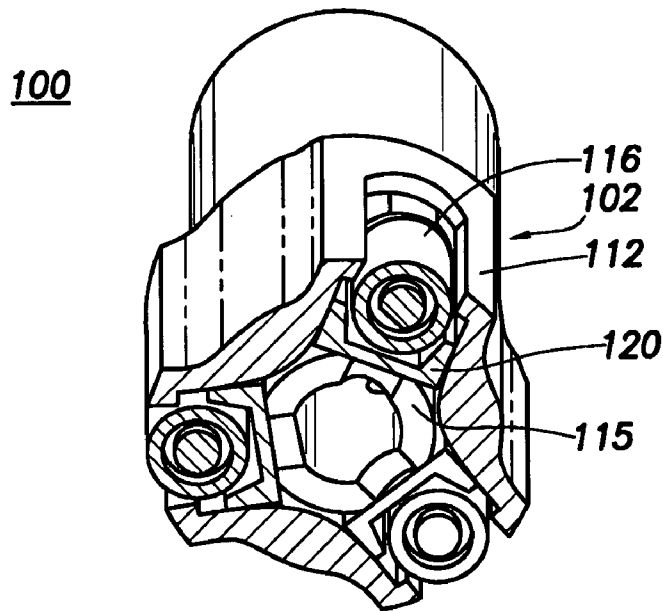
FIG. 2 (PRIOR ART)
