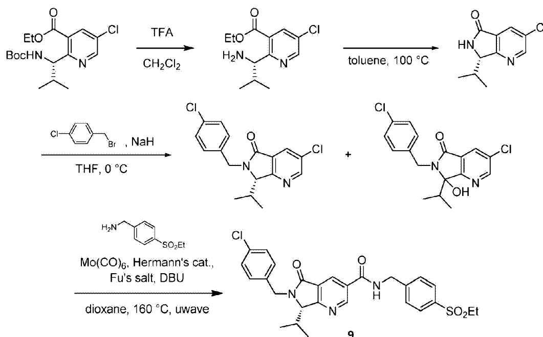
Scheme 13.
