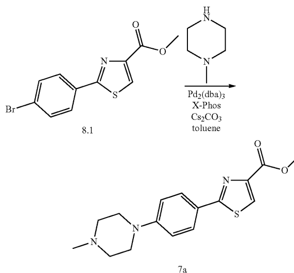
Scheme 8: Synthesis of intermediate 7a
