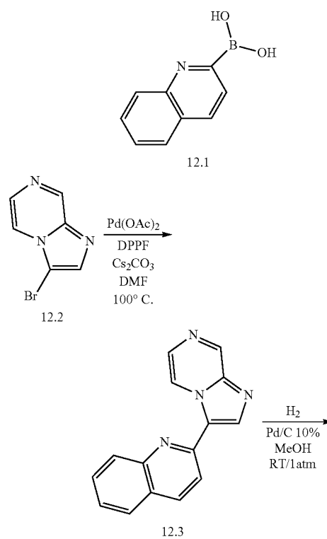
Scheme 11: Synthesis of compound n° 293
