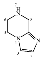
5,6,7,8-tetrahydroimidazo [1,2-a]pyrazine
