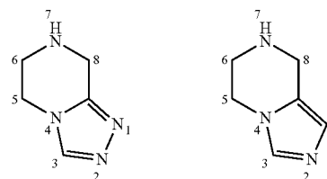
5,6,7,8-tetrahydro-[1,2,4]triazolo [4,3-a]pyrazine 5,6,7,8-tetrahydroimidazo [1,5-a]pyrazine
