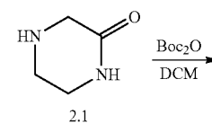
Scheme 2: Synthesis of tert-butyl 3-ethoxy-5,6-dihydropyrazine-1(2H)-carboxylate
