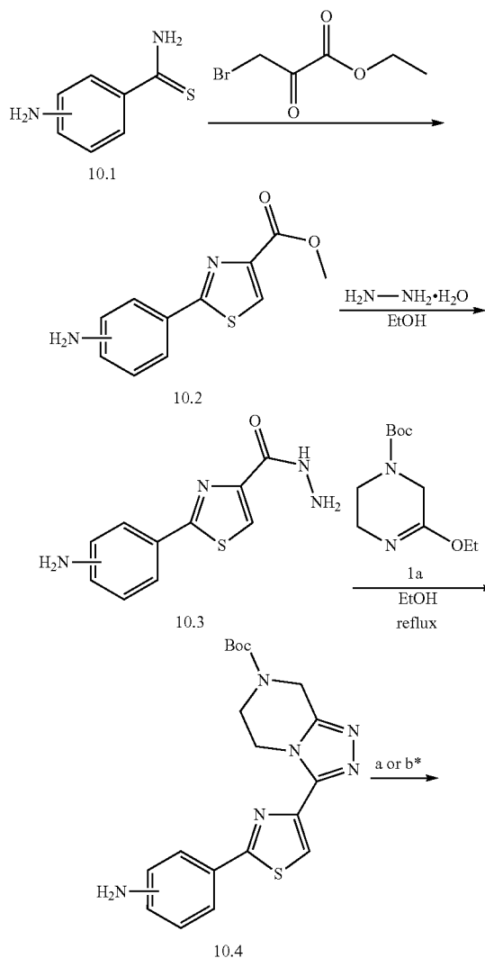
Scheme 10: Synthesis of compounds n° 283, 289, 290, 291, 292
