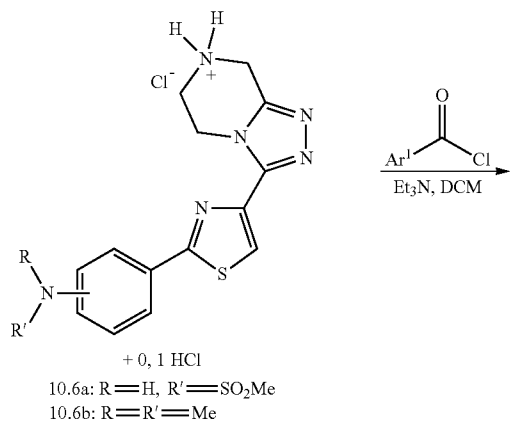
Scheme 10: Synthesis of compounds n° 283, 289, 290, 291, 292
