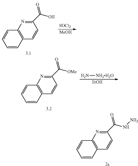
Scheme 3: Synthesis of quinoline-2-carbohydrazide 2a
