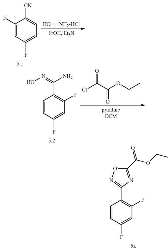
Scheme 6: synthesis of intermediate 5a
