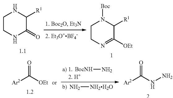
Scheme 1: General synthetic scheme for the preparation of the majority of compounds in the present invention
