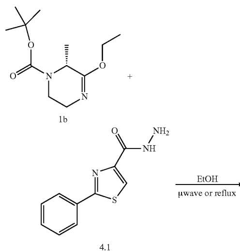
Scheme 4: Synthesis of (R)-4-(8-methyl-5,6,7,8-tetrahydro-[1,2,4]triazolo[4,3-a]pyrazin-3-yl)-2-phenylthiazole hydrochloride salt
