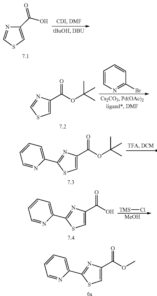
Scheme 7: Synthesis of intermediate 6a
