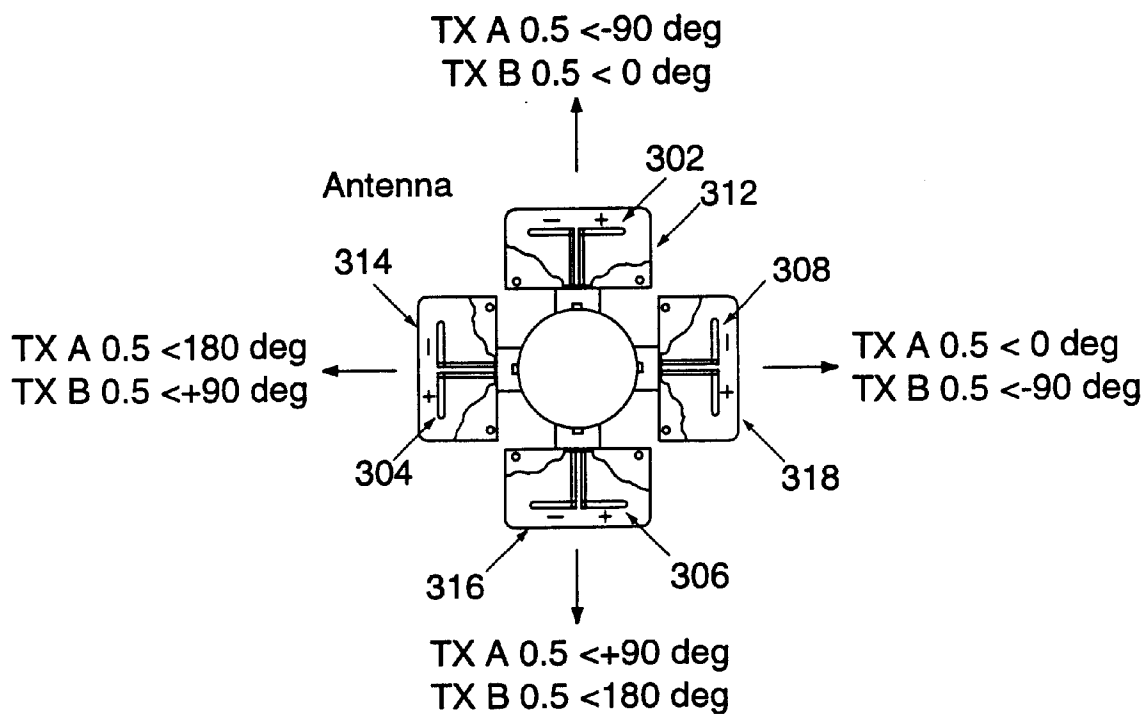
Figure 3. Dipole Panel Antenna Feed with Two Orthogonal Modes
