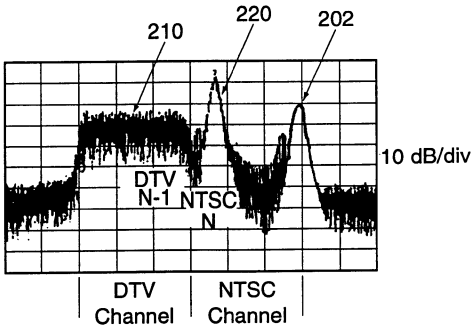
Figure 2A: N-1 Lower Adjacent
