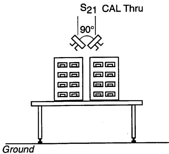
Figure 6. Isolation Between Orthogonal Panel Antennas
