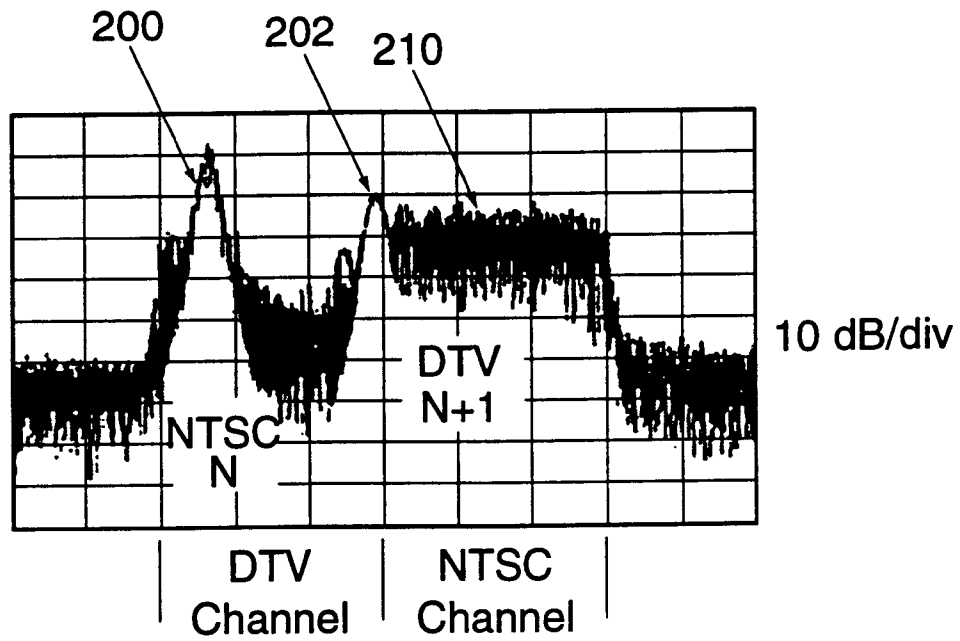
Figure 2B: N+1 Lower Adjacent
