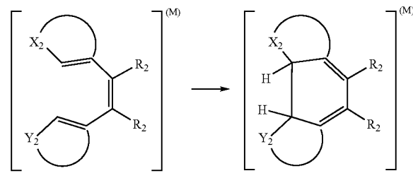
Reaction formula (1)
