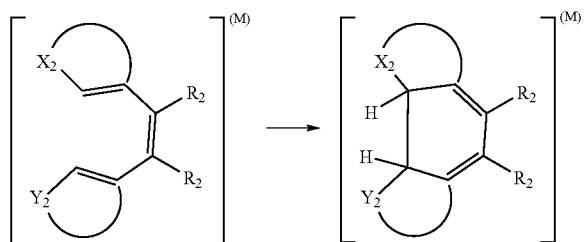
Reaction formula (1)
