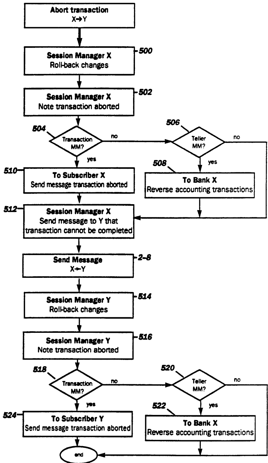
Abort Transaction Money Module to Money Module
