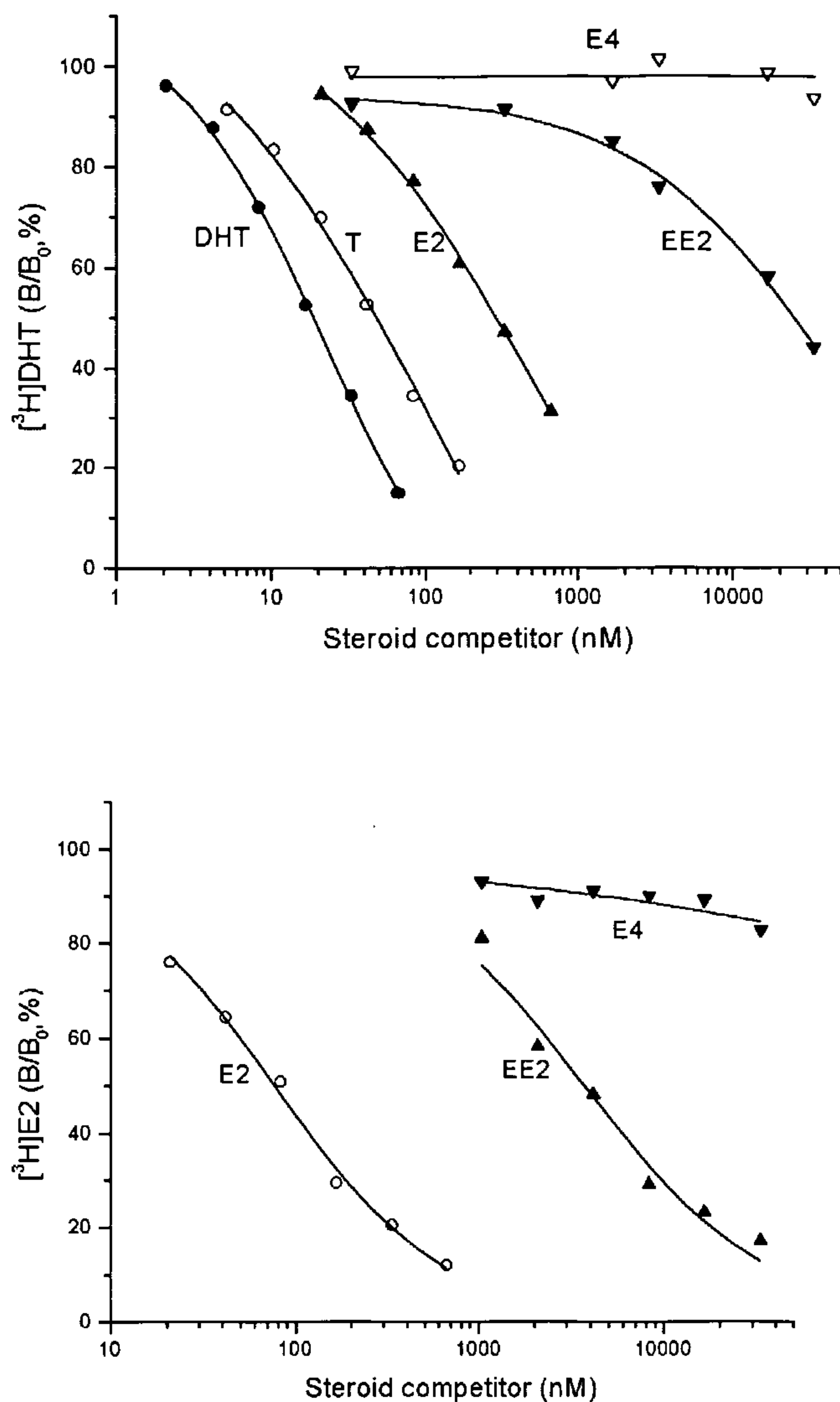
Figure 4: Competitive displacement of [ 3 H]DHT (panel A) and [ 3 H]estradiol (panel B) from the human sex hormone-binding globulin steroid binding site. The unlabeled steroid ligands used as competitors were as follows: estetrol (E4), 17 \alpha -ethinylestradiol (EE2), 17 \beta -estradiol (E2), testosterone (T) and 5 \alpha -dihydrotestosterone (DHT)
