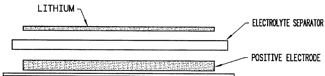
SCHEMATIC OF A L1/ELECTROLYTE SEPARATOR/SULFUR ELECTRODE CELL.
