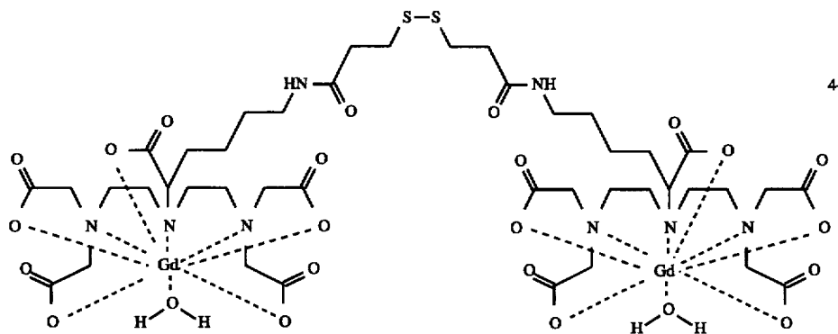
Prototypical Gd complex incorporating the disulfide moiety.
