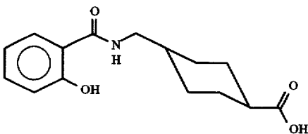
trans-4-(N-salicyloylaminomethyl)cyclohexane carboxylic acid
