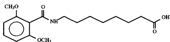
8-(N-2,6-Dimethoxybenzoyl)aminocaprylic acid
