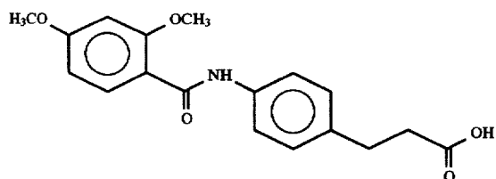
3-[4-(2,4-dimethoxybenzoyl)aminophenyl] propionic acid
