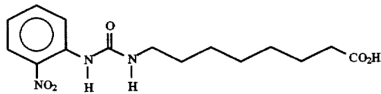
N-2-nitrophenyl-N'-(8-octanoic acid) urea
