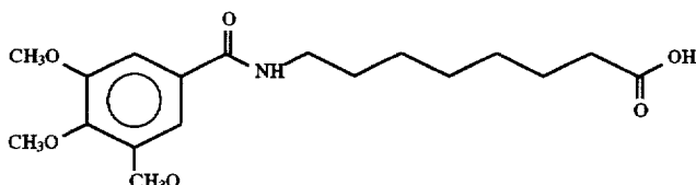
8-(3,4,5-Trimethoxybenzoyl)aminocaprylic acid
