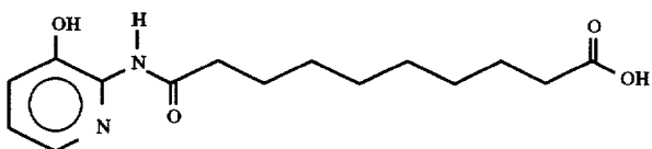
9-[2-(3-hydroxy)pyridylaminocarbonyl]nonanoic acid
