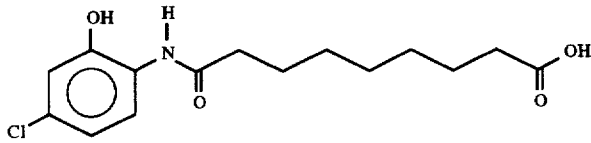
8-(2-hydroxy-5-chloroaminocarbonyl)octanoic acid
