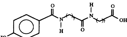
8-(N-(4-Hydroxybenzoyl)]aminocaprylic acid (dimer)
