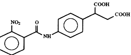
4-(2-Nitrobenzoyl)aminophenylsuccinic acid
