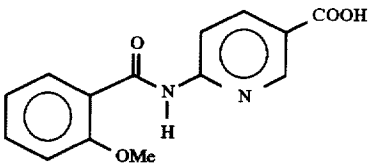
6-(2-methoxybenzoyl)amino nicotinic acid
