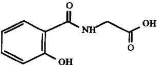
salicyloylglycine
