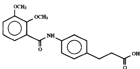
3-[4-(2,3-dimethoxybenzoyl)aminophenyl] propionic acid
