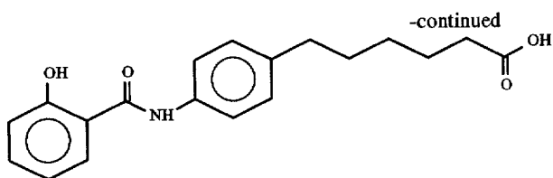
6-(4-salicyloyl)aminophenyl)hexanoic acid
