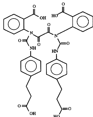
Bis(N-2-carboxyphenyl-N-(N'-3(4-aminophenyl)propionic acid)urea)oxalylyl diamide
