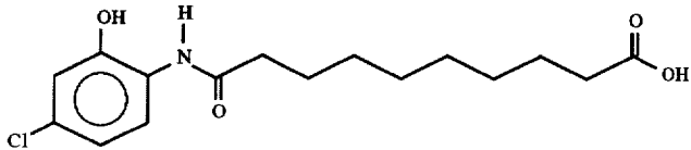
10-(4-chloro-2-hydroxyanilino)sebacic acid monoamide
