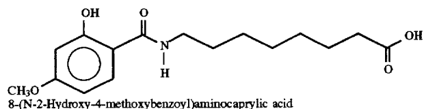
8-(N-(2-Hydroxy-4-methoxybenzoyl)aminocaprylic acid
