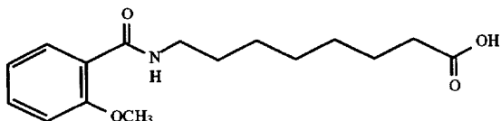
8-(2-methoxybenzoyl)amino caprylic acid
