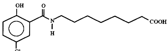
8-(N-2-hydroxy-5-chlorobenzoyl)aminocaproic acid
