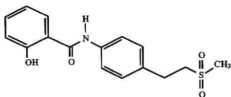
2-[4-Salicyloylamino)phenyl]ethyl methyl sulfone
