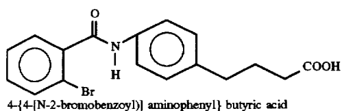
4-[4-[N-(2-bromobenzoyl)]aminophenyl] butyric acid
