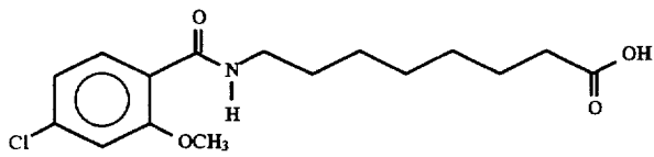
8-(4-chloro-o-anisoyl)aminocaprylic acid
