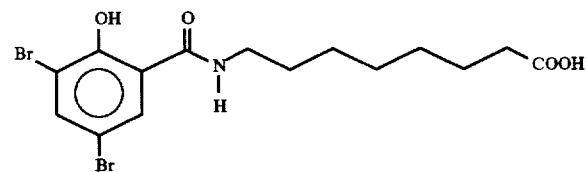
8-[N-(2-acetoxy-3,5-dibromobenzoyl)]aminocaprylic acid
