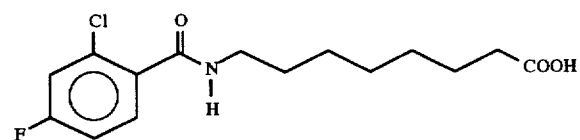
8-(N-(2-chloro-4-fluorobenzoyl)aminocaprylic acid
