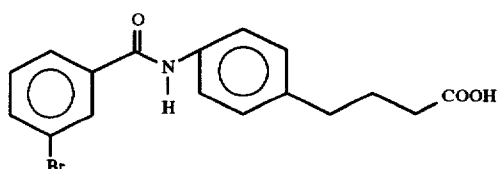
4-[4-[N-(3-bromobenzoyl)]aminophenyl] butyric acid
