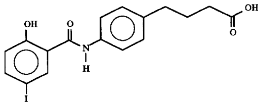
4-[N-(2-hydroxy-5-iodobenzoyl)]aminophenylbutyric acid
