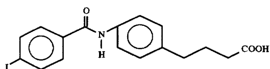
4-[4-[N-(4-iodobenzoyl)]aminophenyl] butyric acid
