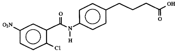
4-(4-(2-chloro-5-nitrobenzoyl)aminophenyl)butyric acid
