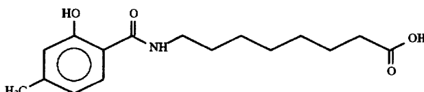
8-(N-4-Methylsalicyloyl)aminocaprillic acid [sic]
