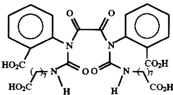
Bis(N-(2-carboxylphenyl)-N-(N'-8-octanoic acid)urea)oxalyl diamide
