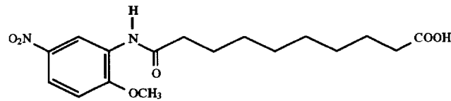
N-(2-methoxy-5-nitrophenyl) sebecoyl amide acid
