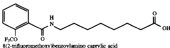
8(2-trifluoromethoxy)benzoylamino caprylic acid
