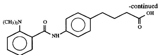
4-(4-(2-Dimethylamino benzoic)aminophenyl)butyric acid
