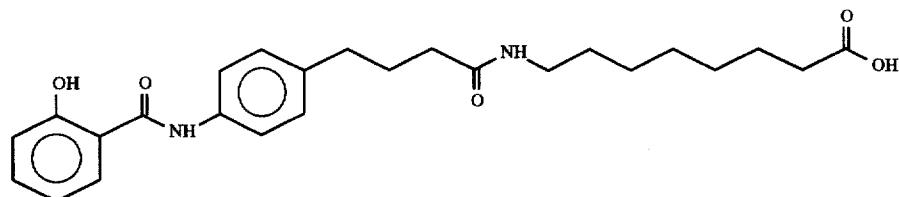
8-(4-(N-Salicyloyl-4aminophenyl)butyric)aminocaprylic acid [sic]
