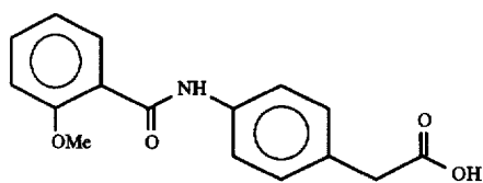
4-(o-anisoyl)aminophenylacetic acid
