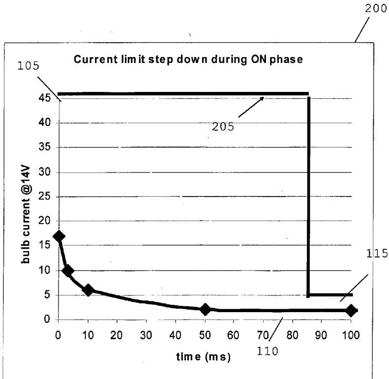
FIG. 2 - Prior art
