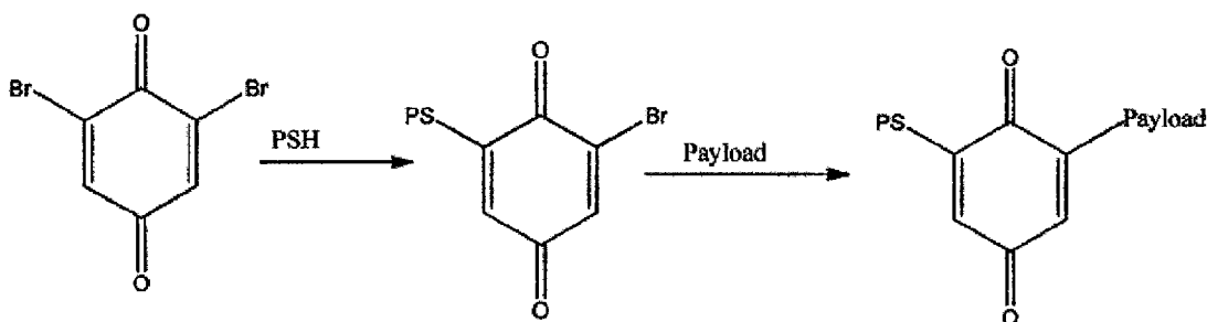
Scheme 23
