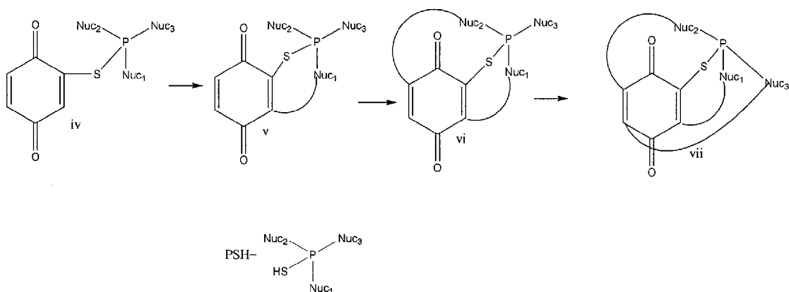
Scheme 15
