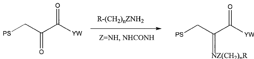
Scheme 28
