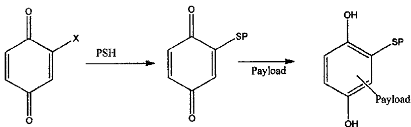
Scheme 22
