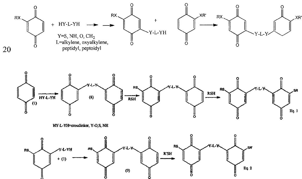
Scheme 24
