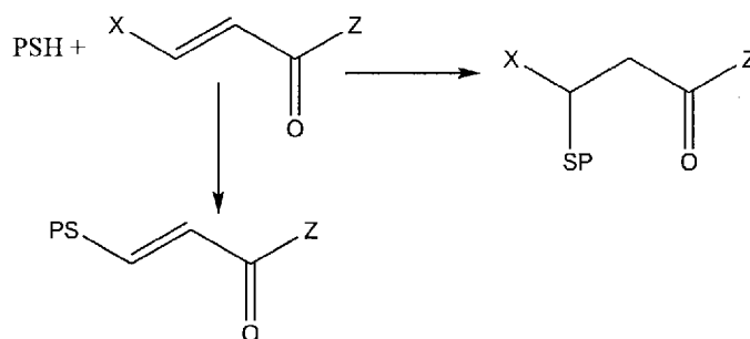
Scheme 30
