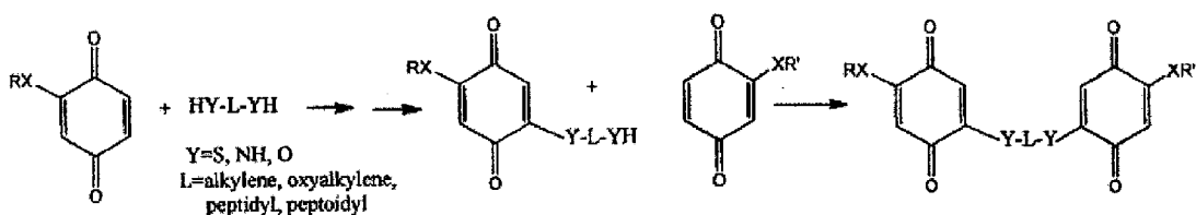
Scheme 16
