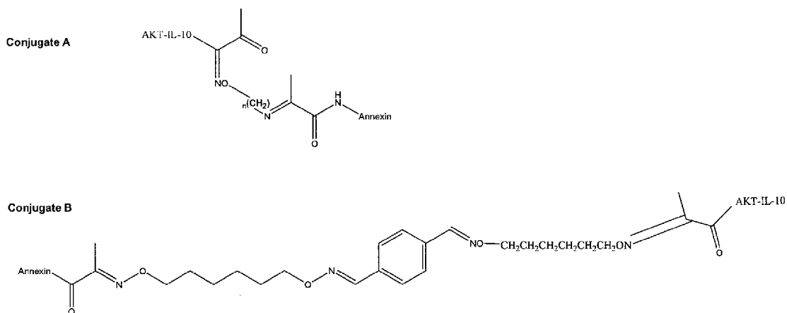
Scheme 35
