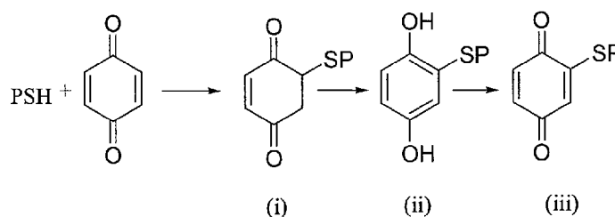
Scheme 13
