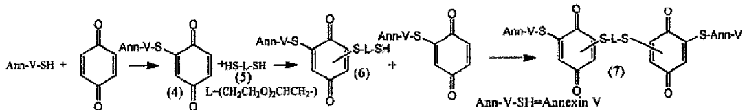
Scheme 19
