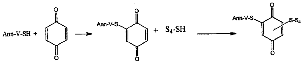
Scheme 17
