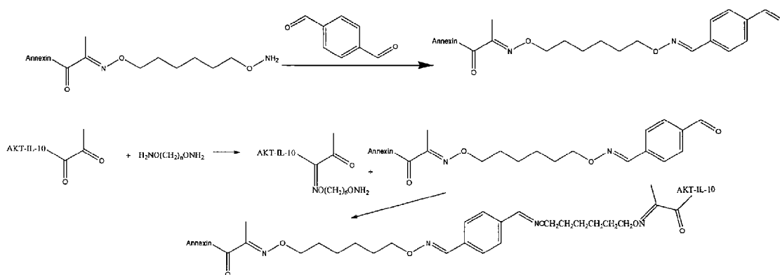
Scheme 34
