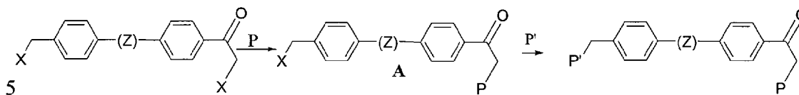
Scheme 9
