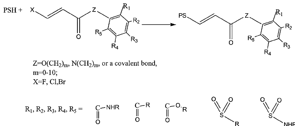
Scheme 31
