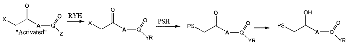
Scheme 12
