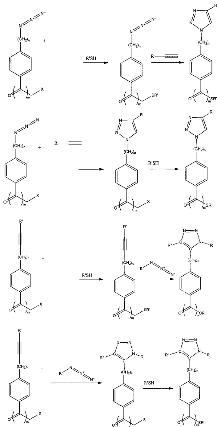
Scheme 10
