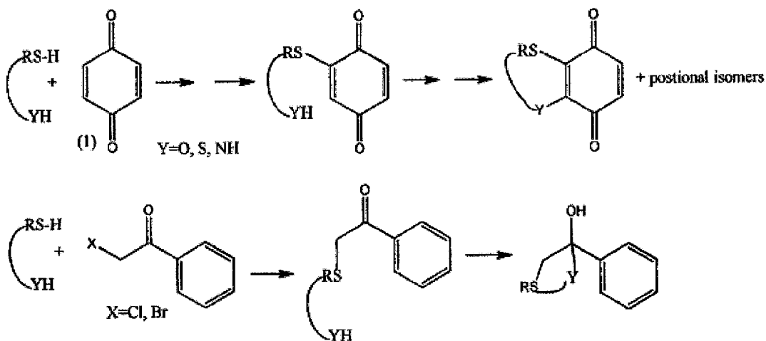
Scheme 14
