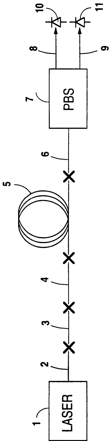
Fig. 1 (PRIOR ART)
