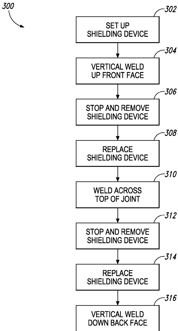
Fig. 3 (Prior Art)
