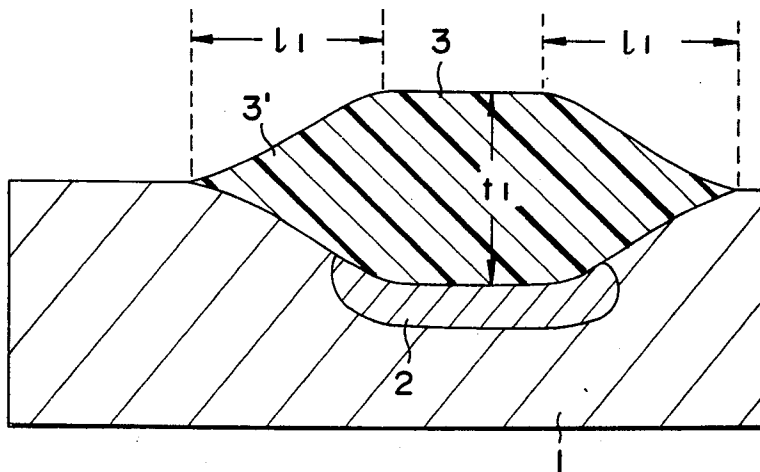
FIG. 2 PRIOR ART
