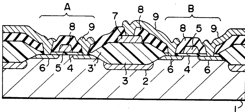
FIG. 1 PRIOR ART
