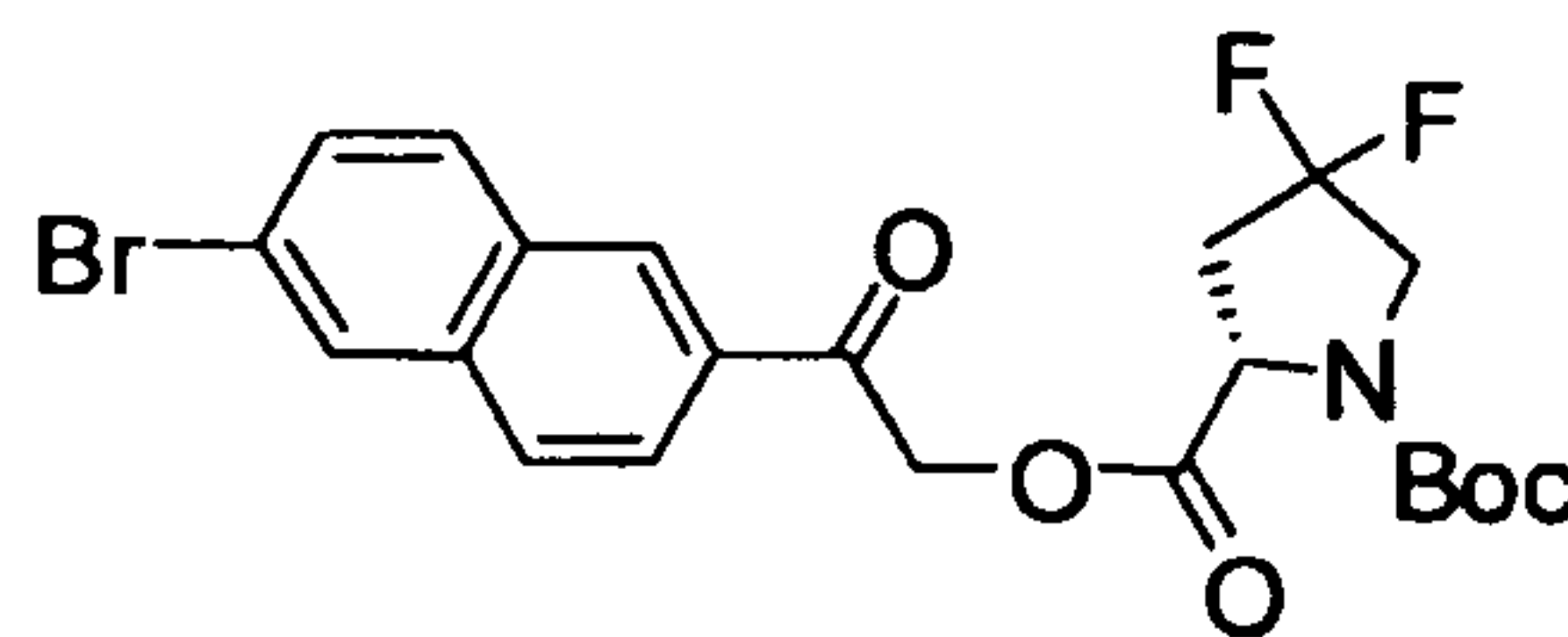
4,4-Difluoro-pyrrolidine-1,2-dicarboxylic acid 2-[2-(6-bromo-naphthalen-2-yl)-2-oxo-ethyl] ester 1- tert -butyl ester
