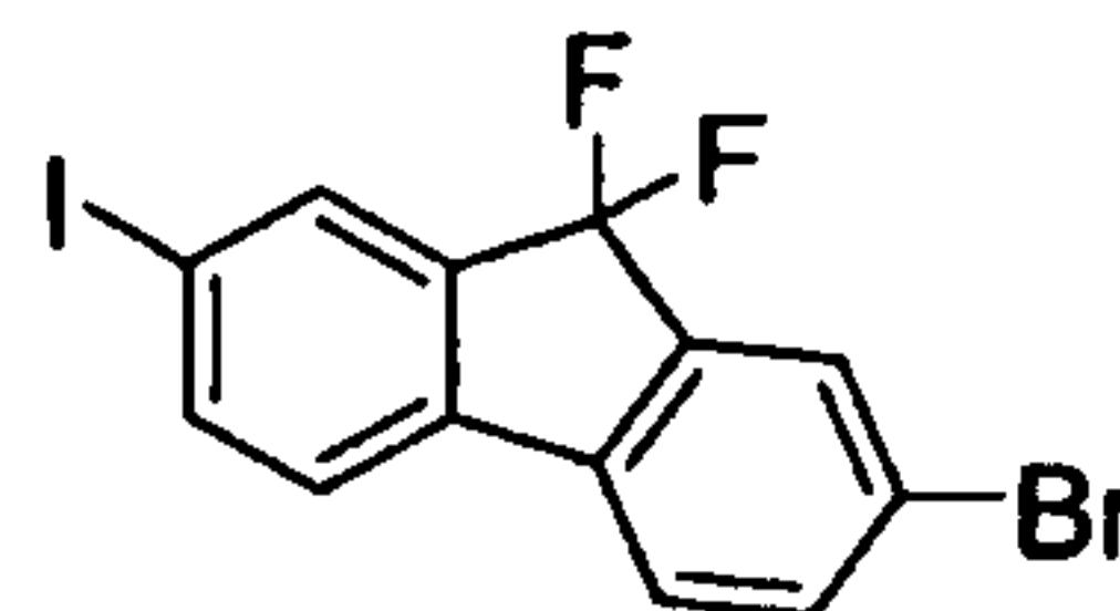
2-Bromo-9,9-difluoro-7-iodo-9H-fluorene
