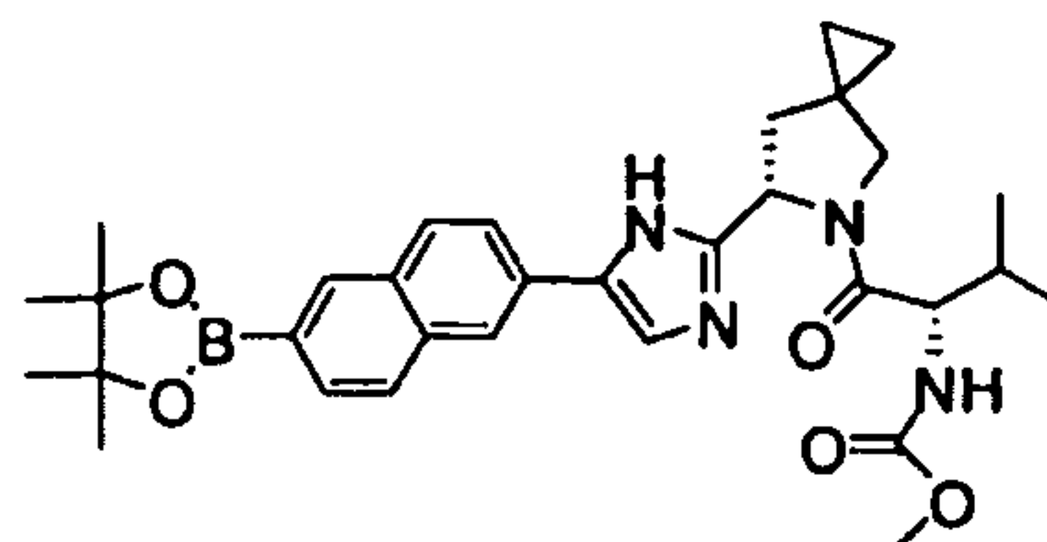
[2-Methyl-1-(6-[5-[6-(4,4,5,5-tetramethyl-[1,3,2]dioxaborolan-2-yl)-naphthalen-2-yl]-1H-imidazol-2-yl]-5-aza-spiro[2.4]heptane-5-carbonyl)-propyl]-carbamic acid methyl ester
