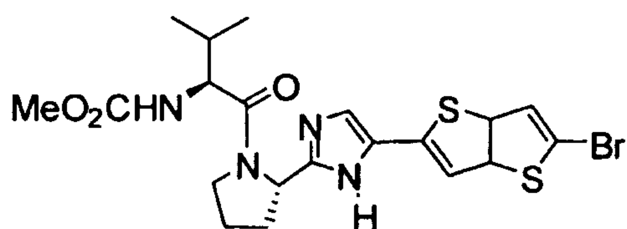
(1-{2-[5-(5-Bromo-3a,6a-dihydro-thieno[3,2- b ]thiophen-2-yl)-1H-imidazol-2-yl]-pyrrolidine-1-carbonyl}-2-methyl-propyl)-carbamic acid methyl ester
