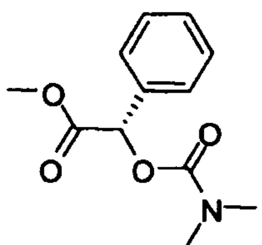
Dimethylcarbamoyloxy-phenyl-acetic acid methyl ester
