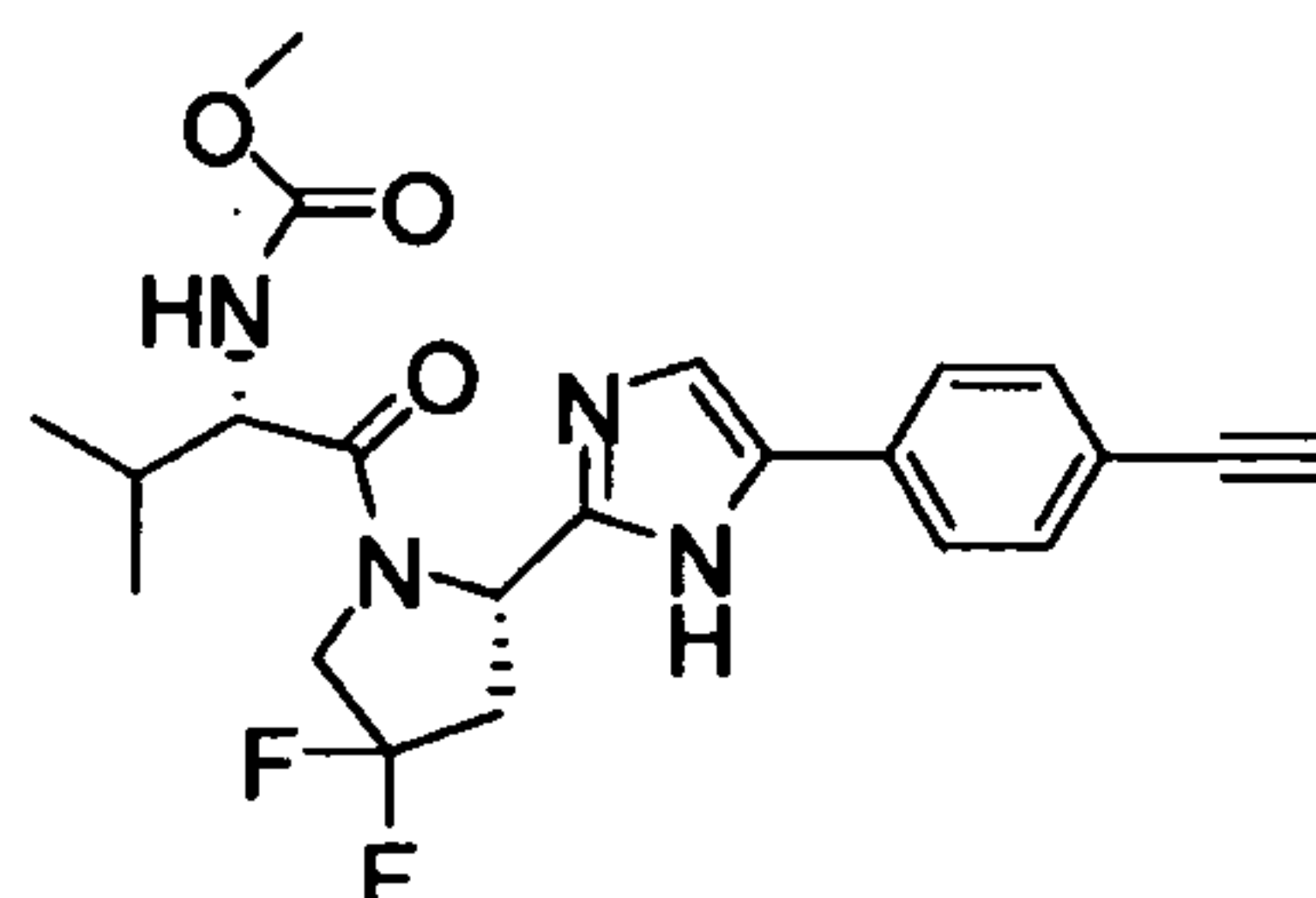
(1-{2-[5-(4-Ethynyl-phenyl)-1H-imidazol-2-yl]-4,4-difluoro-pyrrolidine-1-carbonyl}-2-methyl-propyl)-carbamic acid methyl ester
