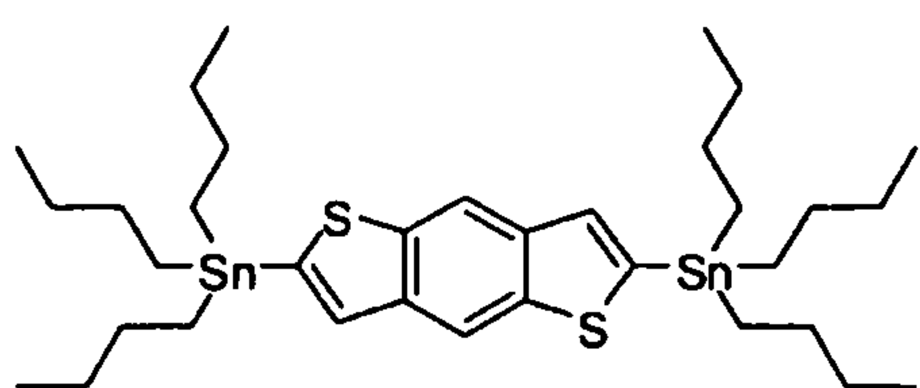
2,6-bis(tri- n -butylstannyl)- benzo[1,2- b :4,5- b' ]dithiophene
