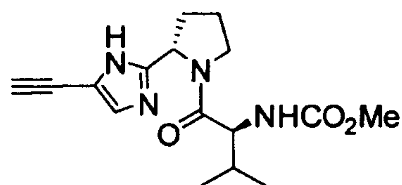
{1-[2-(5-Ethynyl-1H-imidazol-2-yl)-pyrrolidine-1-carbonyl]-2-methyl-propyl}-carbamic acid methyl ester
