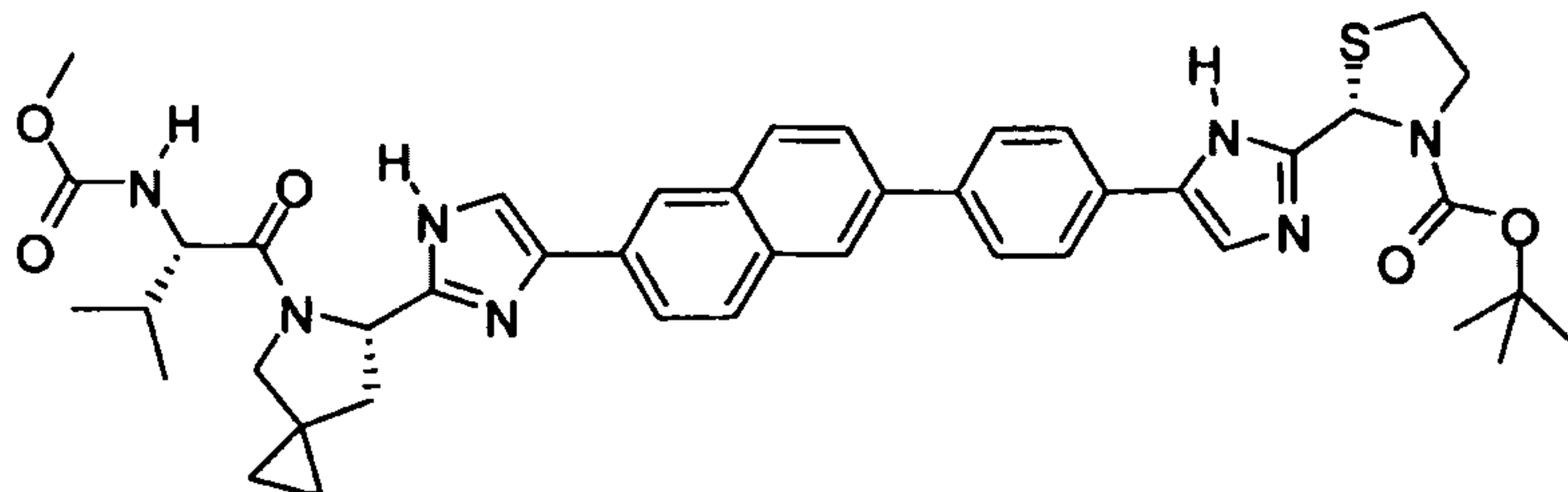
2-[5-[4-(6-[2-[5-(2-Methoxycarbonylamino-3-methyl-butyl)-5-aza-spiro[2.4]hept-6-yl]-1 H -imidazol-4-yl)-naphthalen-2-yl]-phenyl]-1 H -imidazol-2-yl]-thiazolidine-3-carboxylic acid tert -butyl ester
