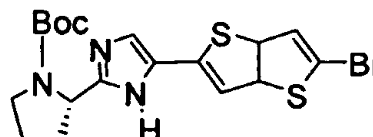
2-[5-(5-Bromo-3a,6a-dihydro-thieno[3,2- b ]thiophen-2-yl)-1H-imidazol-2-yl]-pyrrolidine-1-carboxylic acid tert -butyl ester
