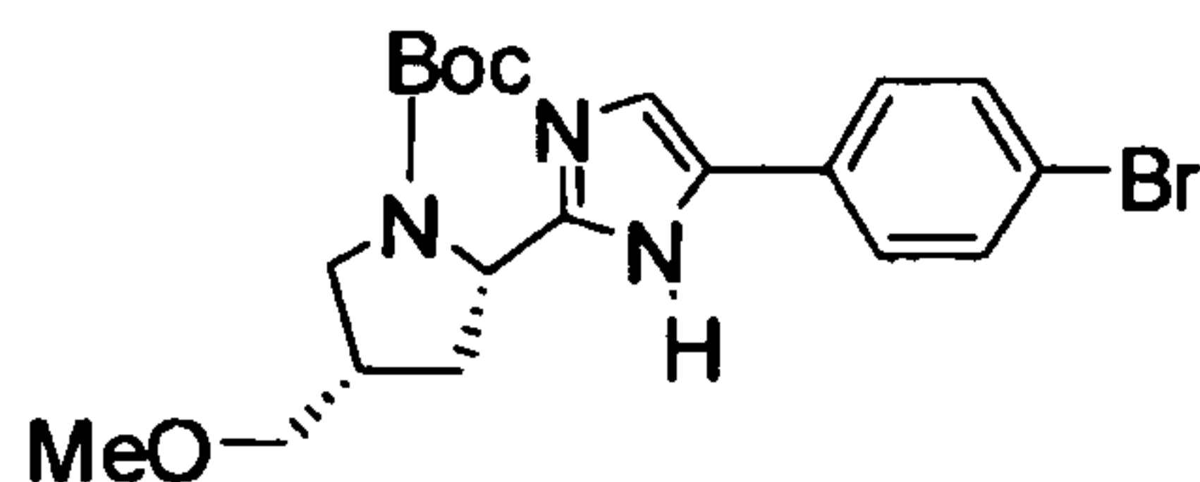
2-[5-(4-Bromo-phenyl)-1 H -imidazol-2-yl]-4-methoxymethyl-pyrrolidine-1-carboxylic acid tert -butyl ester
