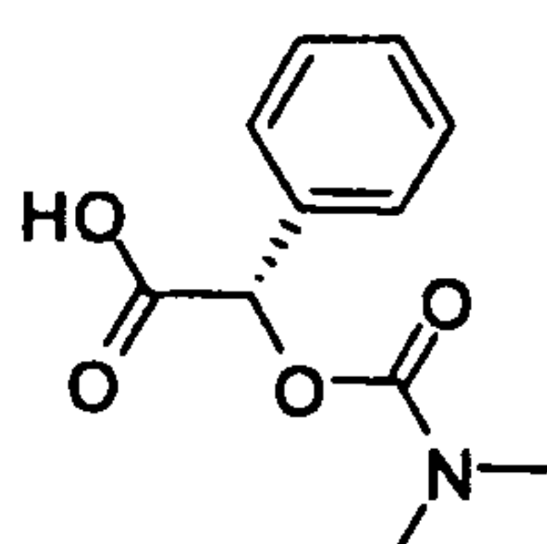
Dimethylcarbamoyloxy-phenyl-acetic acid
