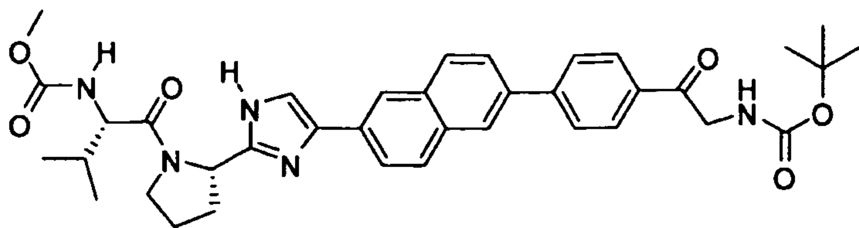
{1-[2-(4-[6-[4-(2- tert -Butoxycarbonylamino-acetyl)-phenyl]-naphthalen-2-yl)-1 H -imidazol-2-yl]-pyrrolidine-1-carbonyl]-2-methyl-propyl}-carbamic acid methyl ester
