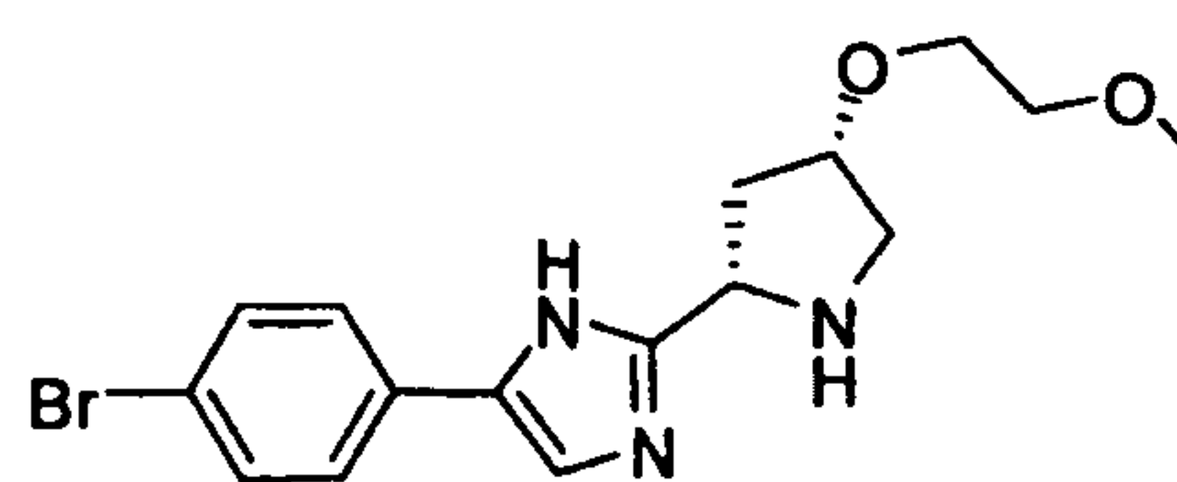
5-(4-Bromo-phenyl)-2-[4-(2-methoxy-ethoxy)-pyrrolidin-2-yl]-1 H -imidazole
