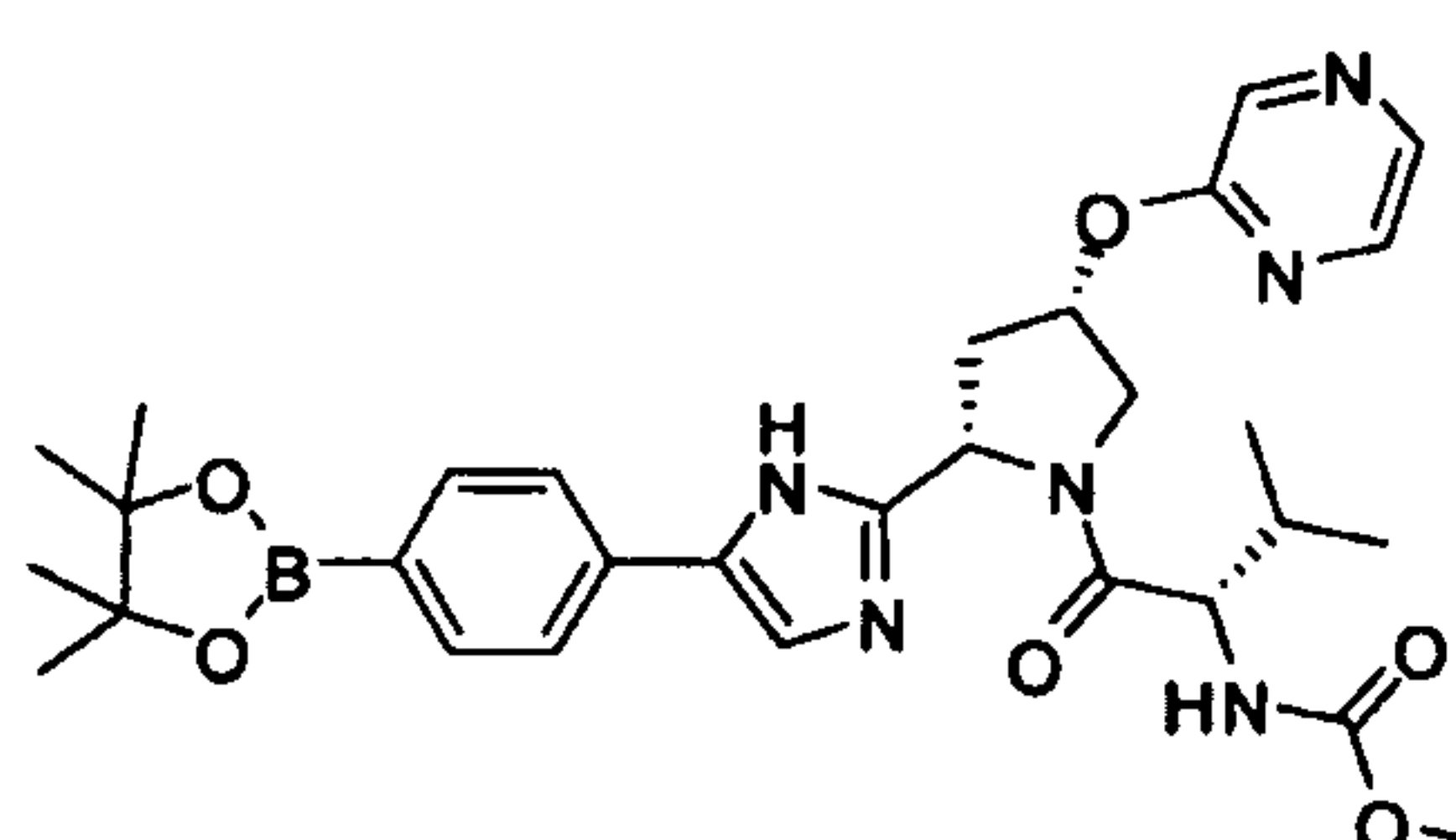
[2-Methyl-1-(4-(pyrazin-2-yloxy)-2-(5-[4-(4,4,5,5-tetramethyl-1,3,2)dioxaborolan-2-yl]-phenyl)-1 H -imidazol-2-yl)-pyrrolidine-1-carbonyl]-propyl]-carbamic acid methyl ester
