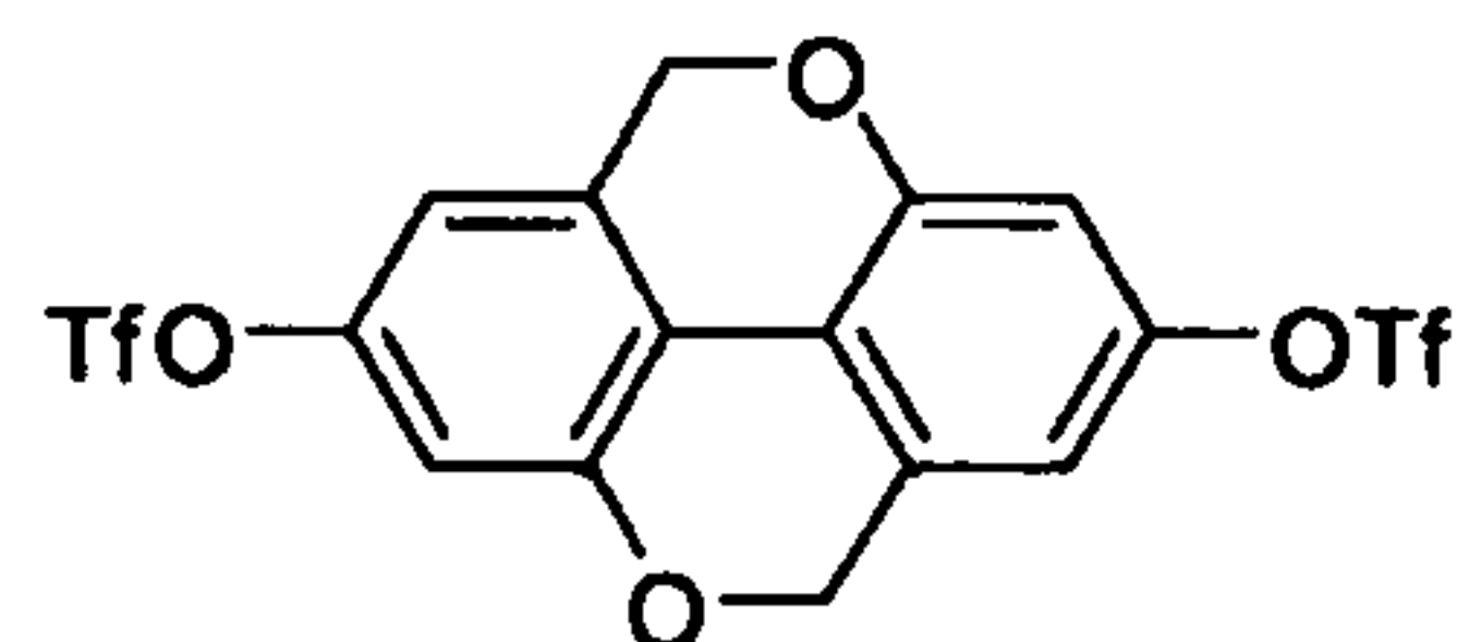
Trifluoro-methanesulfonic acid 7-trifluoro methanesulfonyloxy-5,10-dihydro-chromeno[5,4,3-cde]chromen-2-yl ester
