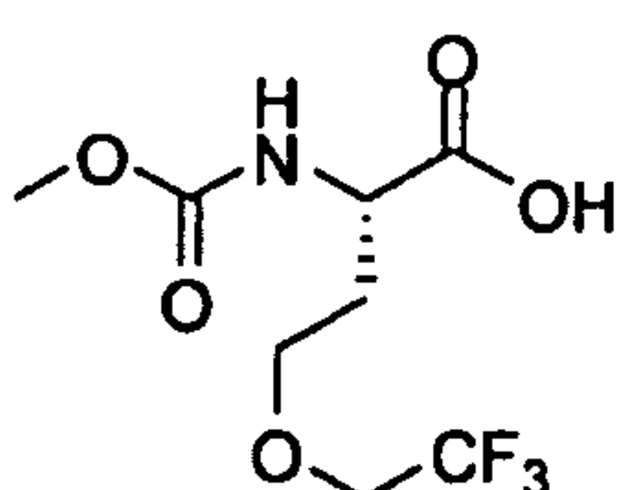
2-Methoxycarbonylamino-4-(2,2,2-trifluoro-ethoxy)-butyric acid
