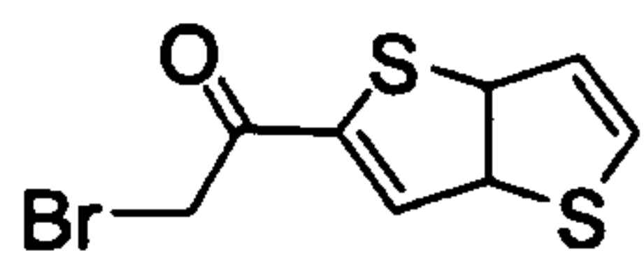
2-Bromo-1-(3a,6a-dihydrothieno[3,2-b]thiophen-2-yl)-ethanone
