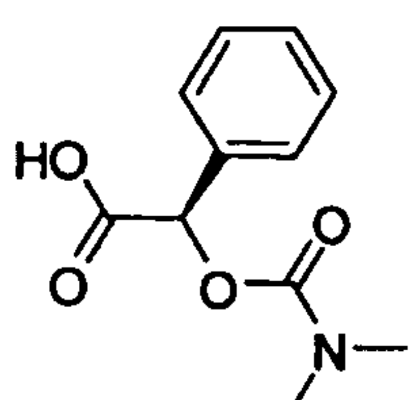
Dimethylcarbamoyloxy-phenyl-acetic acid
