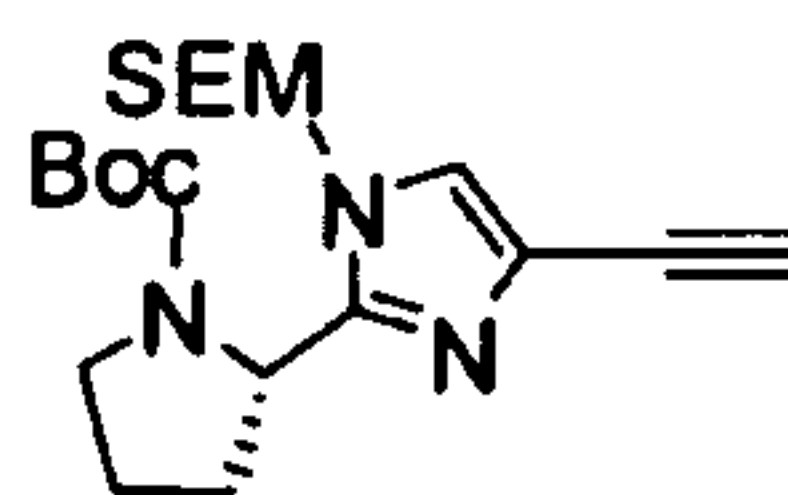
2-[4-Ethynyl-1-(2-trimethylsilyl-ethoxymethyl)-1H-imidazol-2-yl]-pyrrolidine-1-carboxylic acid tert -butyl ester
