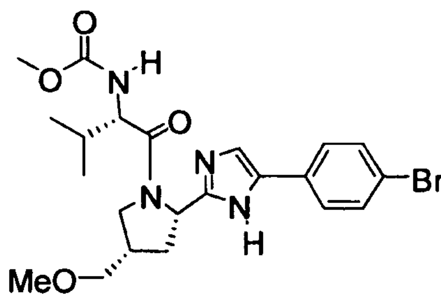
(1-{2-[5-(4-Bromo-phenyl)-1 H -imidazol-2-yl]-4-methoxymethyl-pyrrolidine-1-carbonyl}-2-methyl-propyl)-carbamic acid methyl ester
