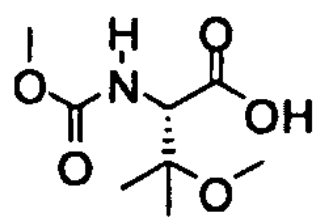
( S )-3-Methoxy-2-methoxycarbonylamino- 3-methylbutyric acid
