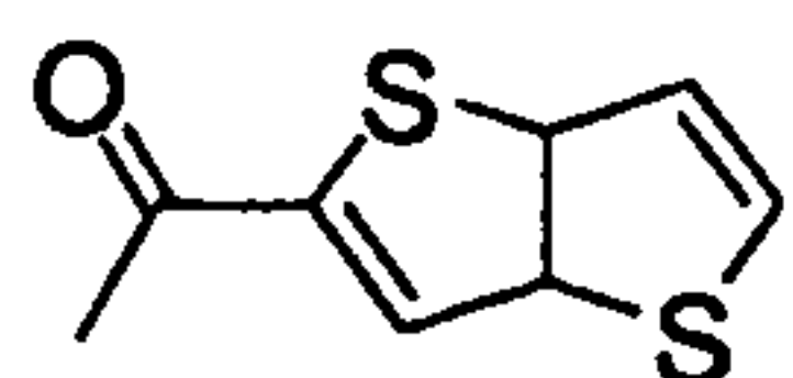
1-(3a,6a-Dihydrothieno[3,2-b]thiophen-2-yl)-ethanone
