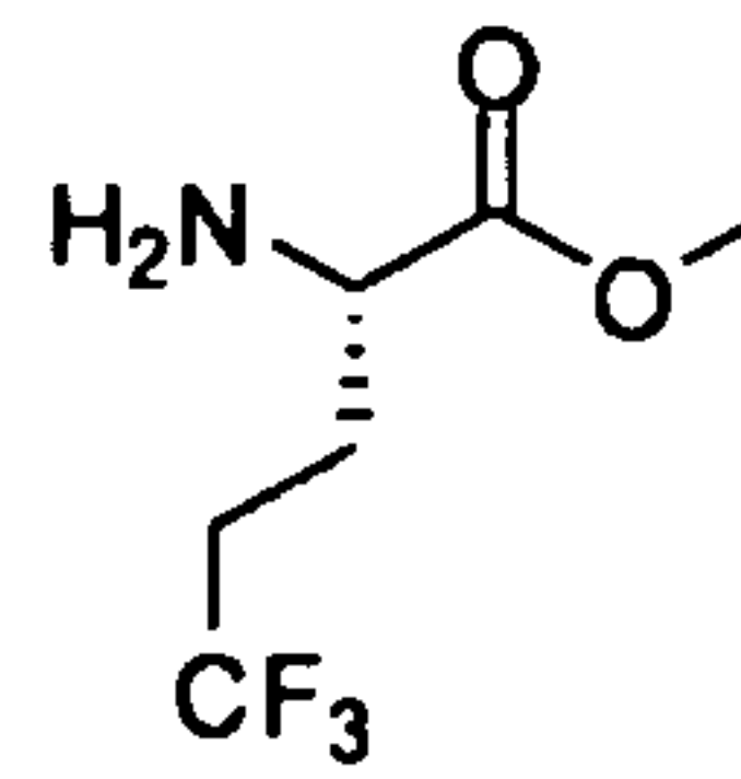
2-Amino-5,5,5-trifluoropentanoic acid methyl ester
