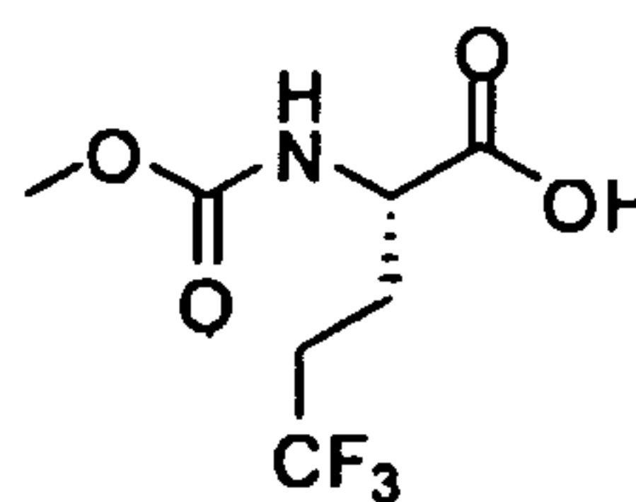
5,5,5-Trifluoro-2-methoxycarbonylamino-pentanoic acid
