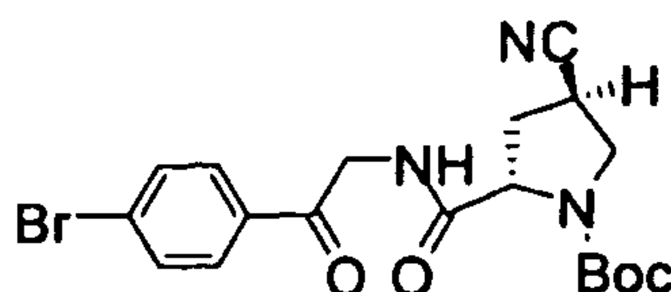
2-[2-(4-Bromo-phenyl)-2-oxoethylcarbamoyl]-4-cyano-pyrrolidine-1-carboxylic acid tert -butyl ester
