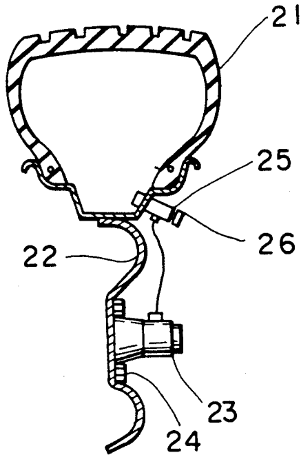
FIG. 8 PRIOR ART
