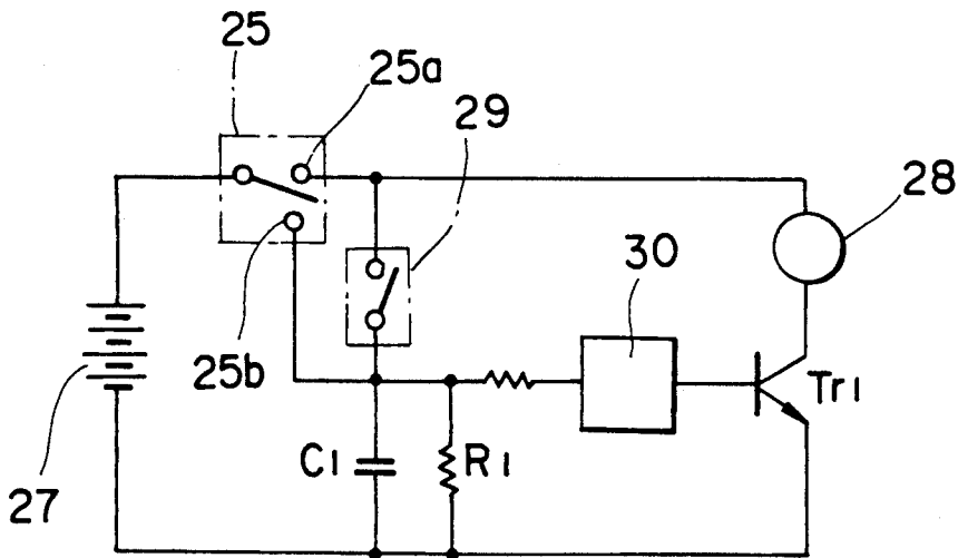
FIG. 9 PRIOR ART
