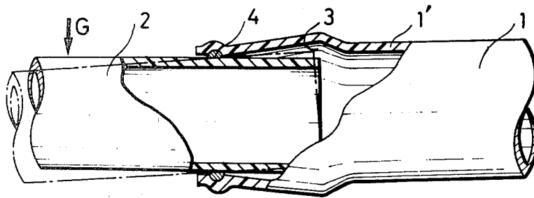
FIG. 1 PRIOR ART
