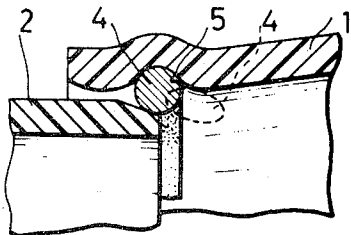
FIG. 2 PRIOR ART
