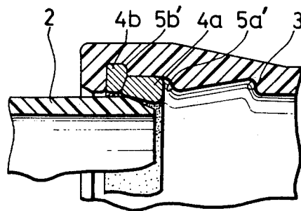
FIG. 5 PRIOR ART
