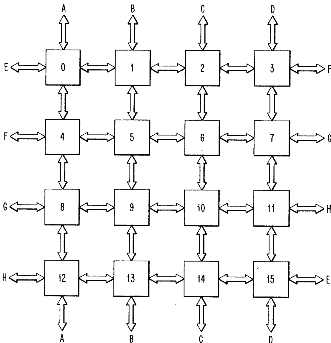
FIG. 2 (PRIOR ART)
