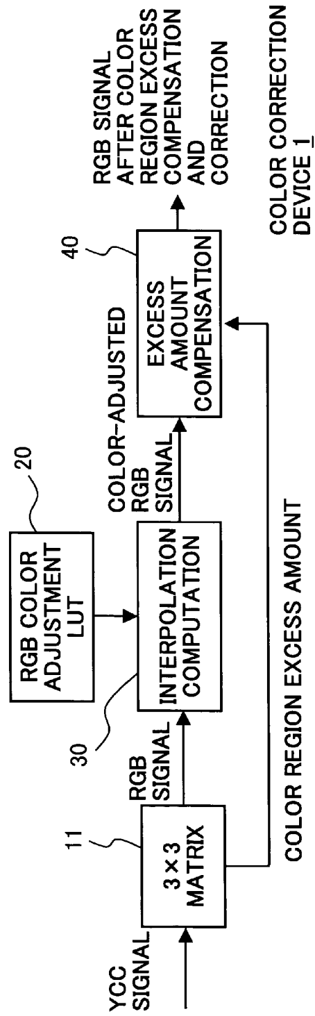
FIG. 1B CONFIGURATION EXAMPLE OF COLOR CORRECTION DEVICE
