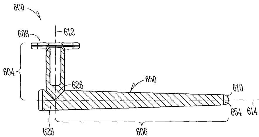
SECTION 6B-6B
