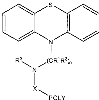
Formula Ia-C
