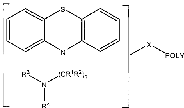
Formula I-C
