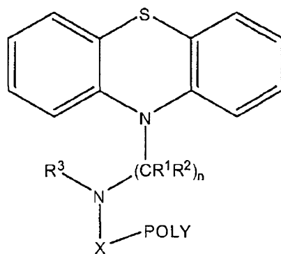
Formula I-C
