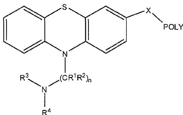
Formula Ib-C
