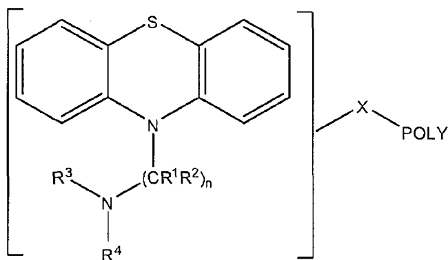
Formula I-C
