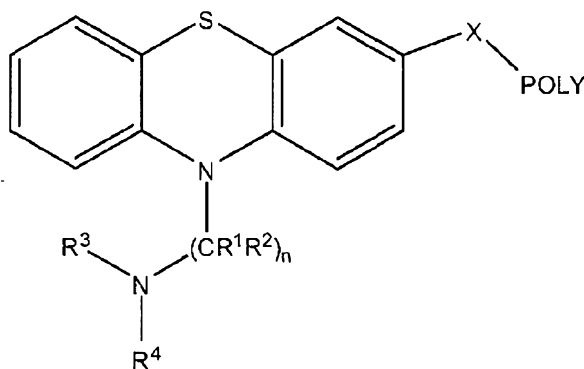
Formula Ib-C
