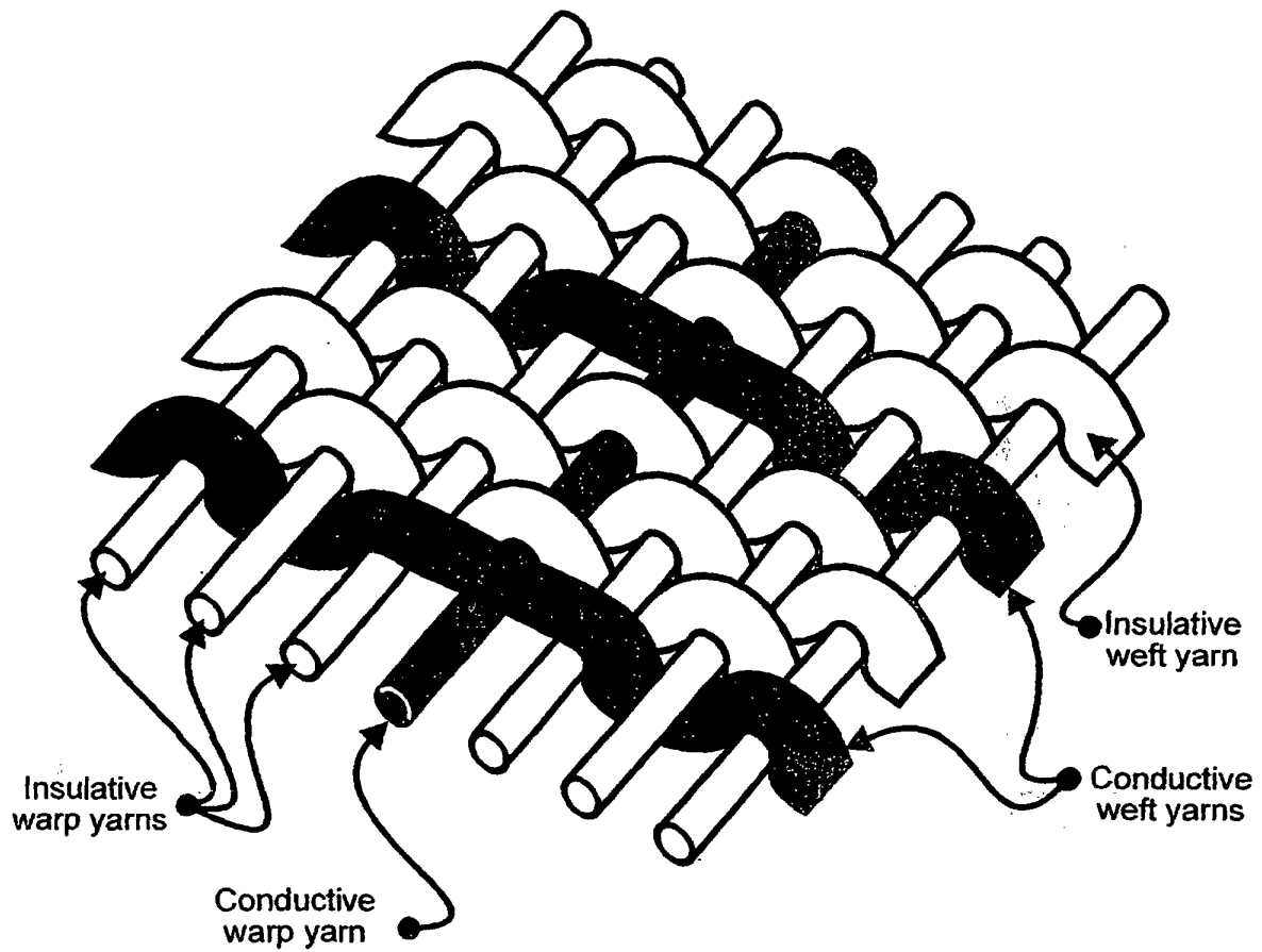
Figure 3. Woven piece of fabric, showing conductive and insulative yarns, with weft floats at crossover points between conductors
