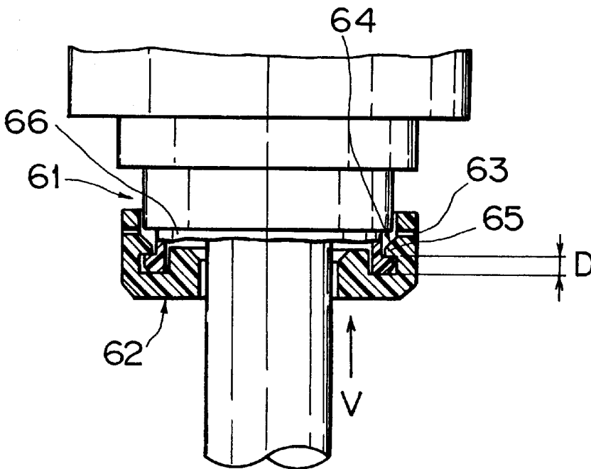
FIG. 8 PRIOR ART
