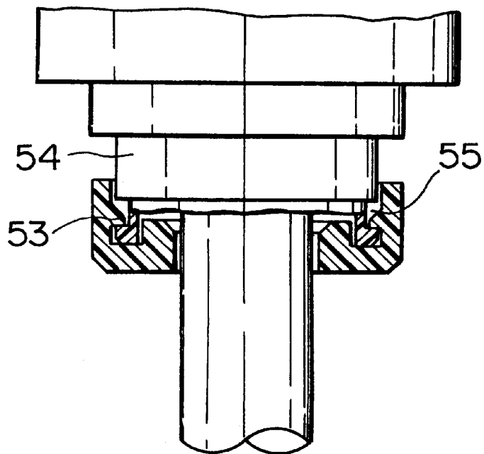
FIG. 6 PRIOR ART
